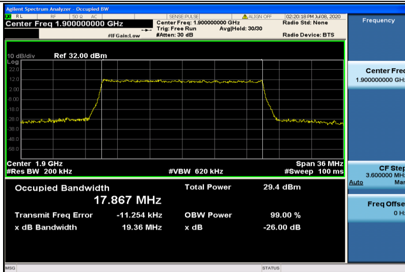
Band2-20MHz-QPSK-19100-100RB#0-17.867
