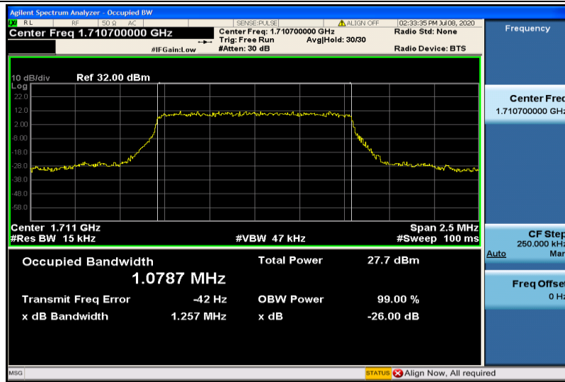
Band4-1.4MHz-QPSK-19957-6RB#0-1.0787
