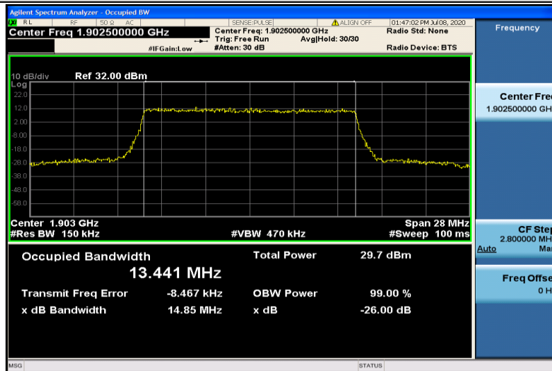
Band2-15MHz-QPSK-19125-75RB#0-13.441
