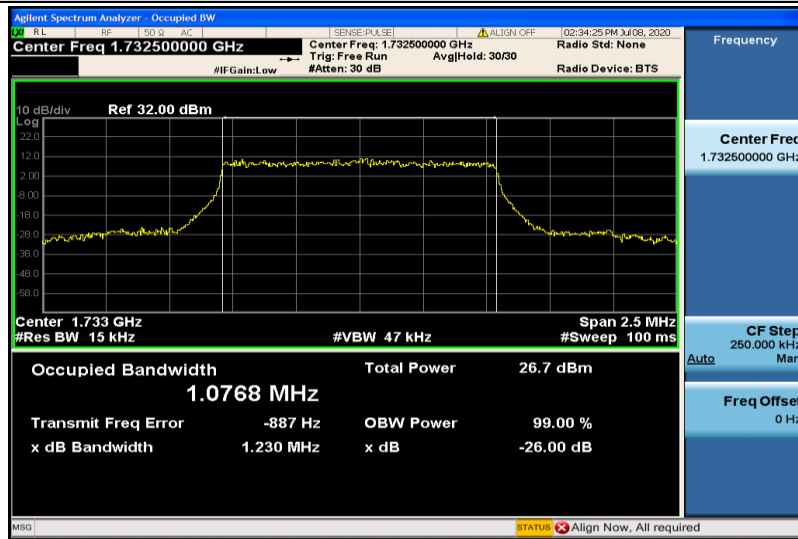
Band4-1.4MHz-16QAM-20175-6RB#0-1.0768
