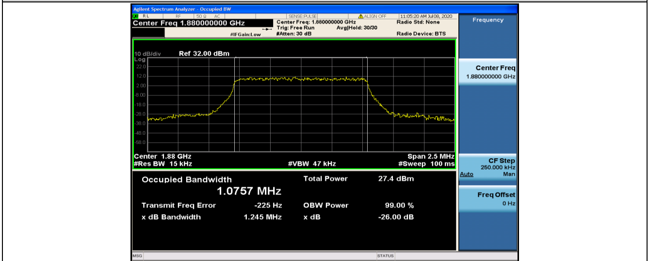
Band2-1.4MHz-QPSK-18900-6RB#0-1.0757
