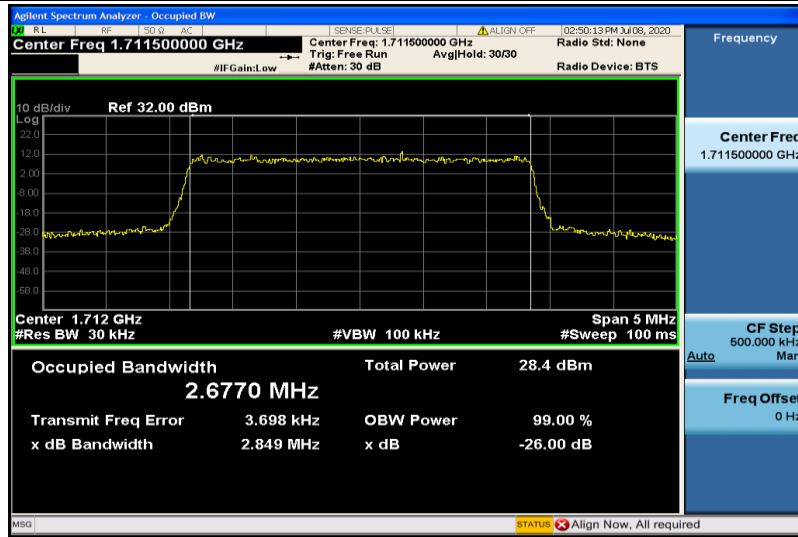
Band4-3MHz-QPSK-19965-15RB#0-2.6770
