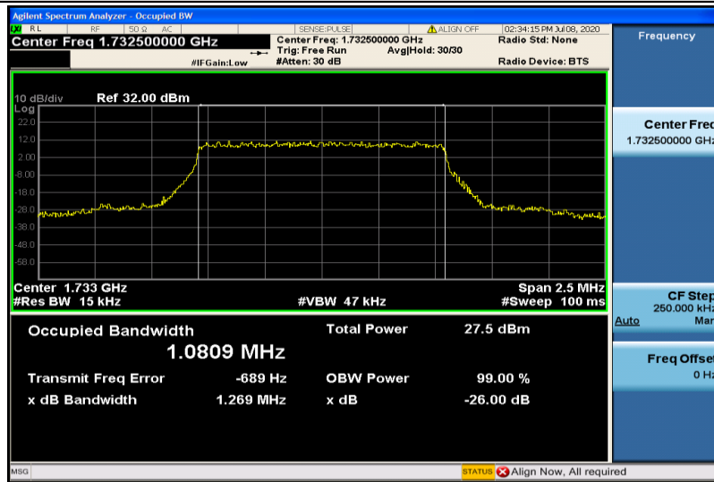
Band4-1.4MHz-QPSK-20175-6RB#0-1.0809
