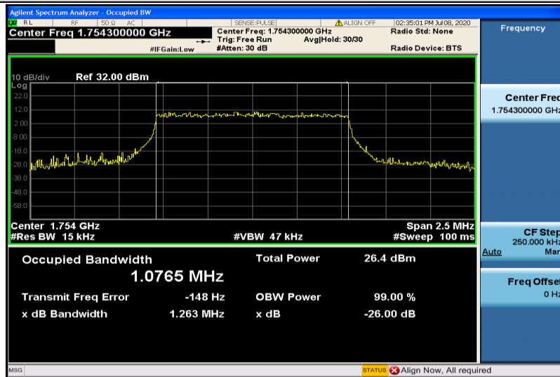
Band4-1.4MHz-16QAM-20393-6RB#0-1.0765
