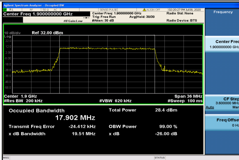
Band2-20MHz-16QAM-19100-100RB#0-17.902
