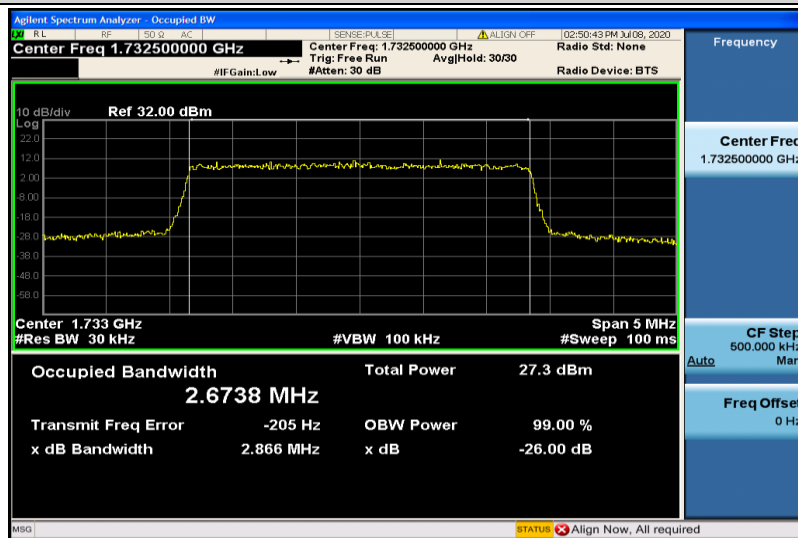
Band4-3MHz-16QAM-20175-15RB#0-2.6738
