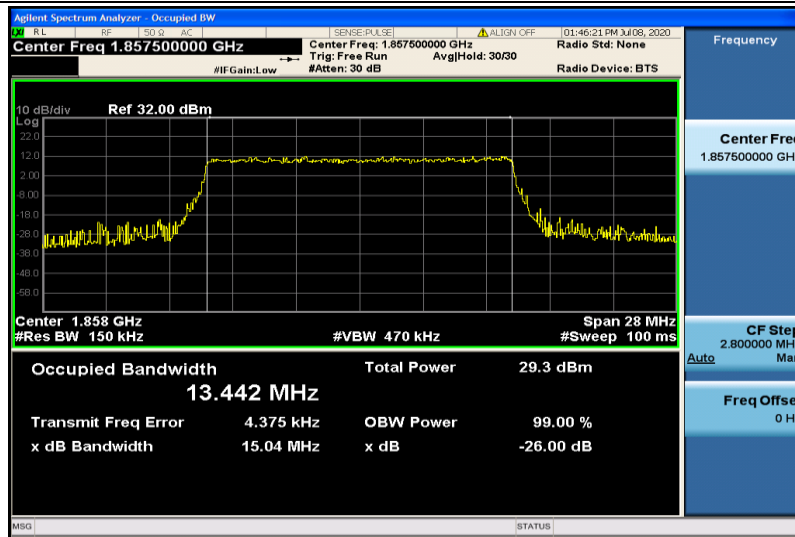
Band2-15MHz-QPSK-18675-75RB#0-13.442
