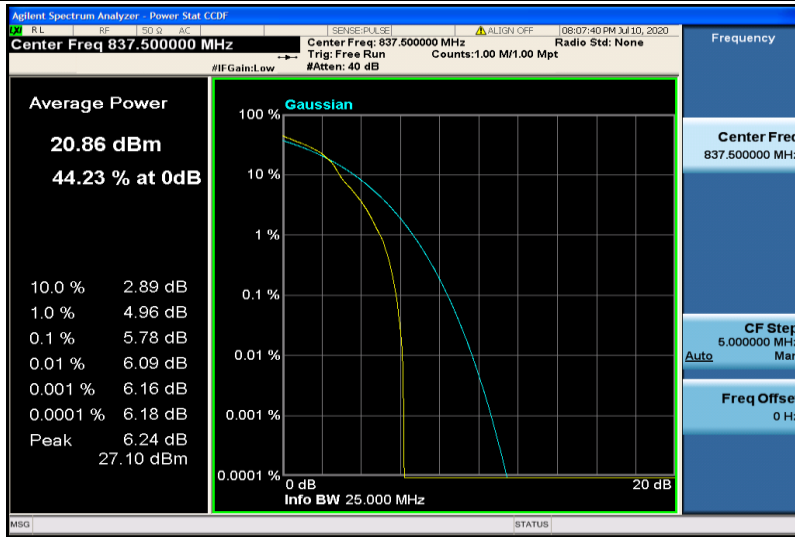
Band19-10MHz-16QAM-24075-1RB#0
