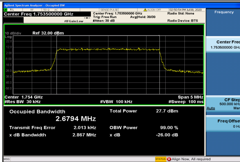
Band4-3MHz-QPSK-20385-15RB#0-2.6794
