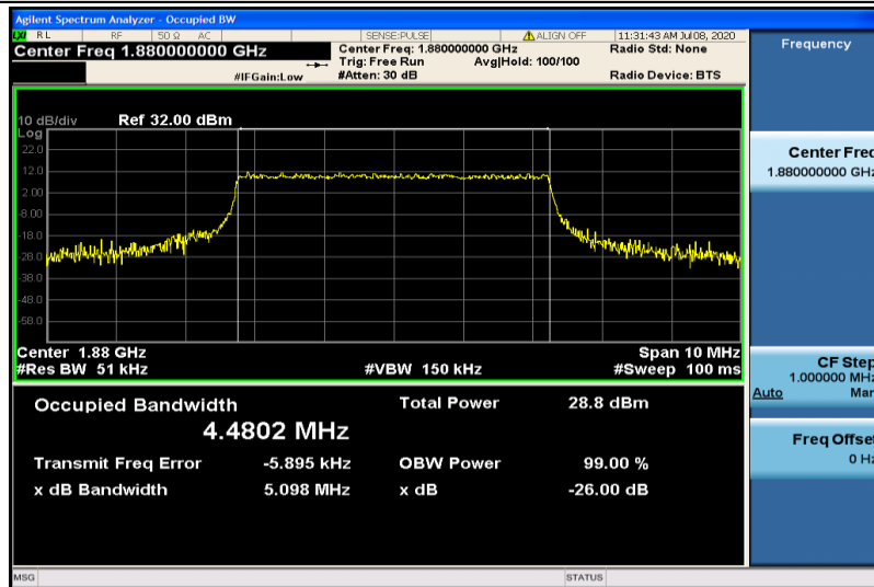
Band2-5MHz-QPSK-18900-25RB#0-4.4802
