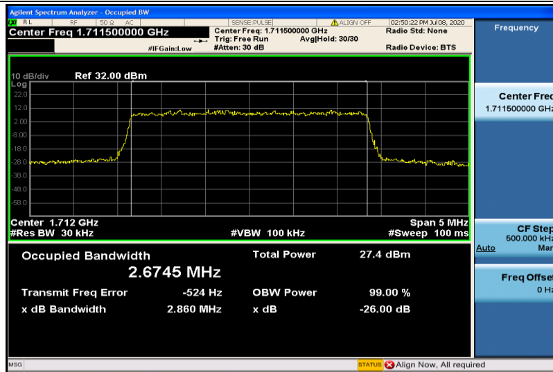
Band4-3MHz-16QAM-19965-15RB#0-2.6745
