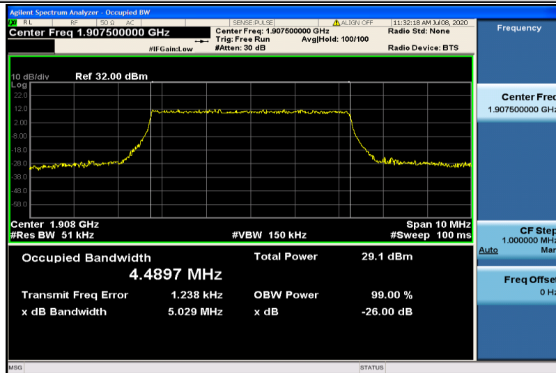
Band2-5MHz-QPSK-19175-25RB#0-4.4897
