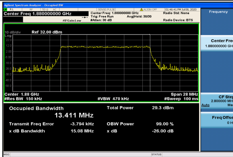
Band2-15MHz-QPSK-18900-75RB#0-13.411
