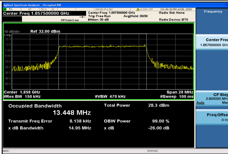
Band2-15MHz-16QAM-18675-75RB#0-13.448
