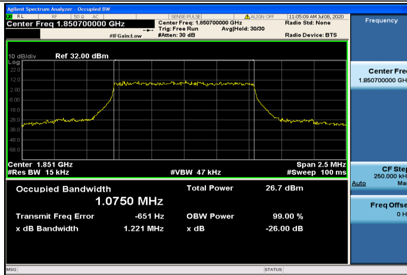
Band2-1.4MHz-16QAM-18607-6RB#0-1.0750
