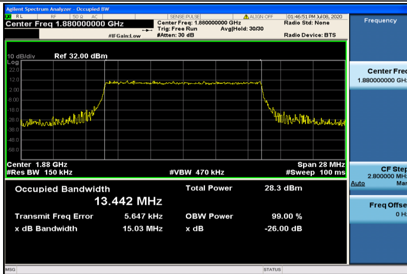
Band2-15MHz-16QAM-18900-75RB#0-13.442
