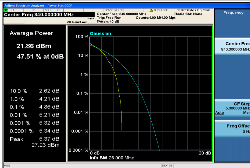
Band19-10MHz-QPSK-24100-1RB#0
