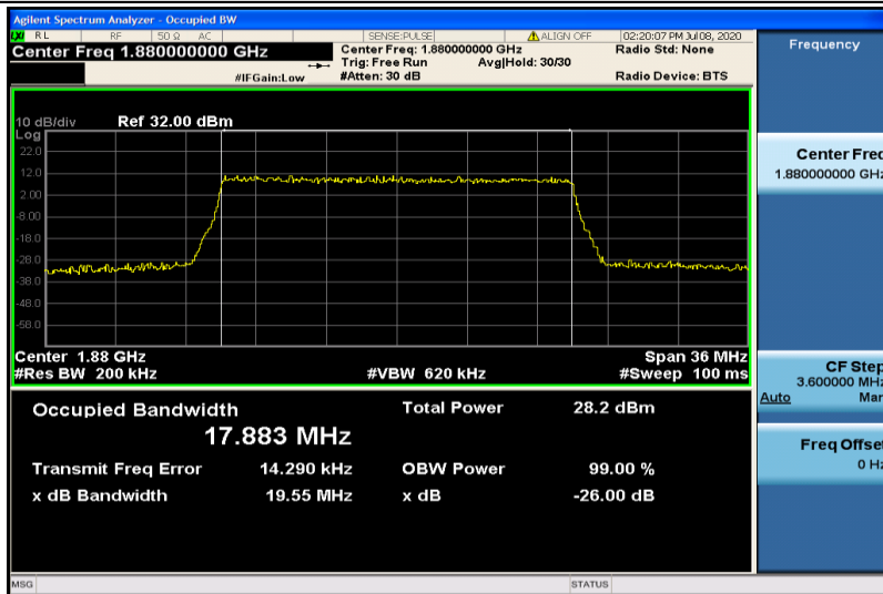
Band2-20MHz-16QAM-18900-100RB#0-17.883
