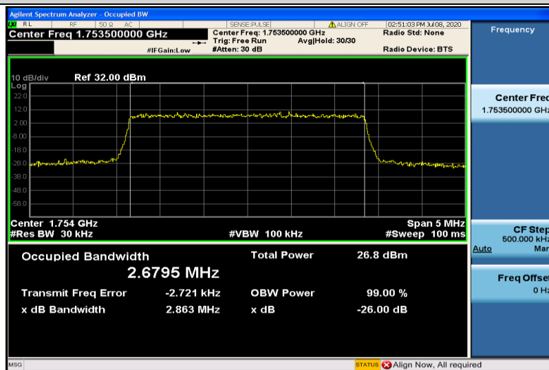
Band4-3MHz-16QAM-20385-15RB#0-2.6795
