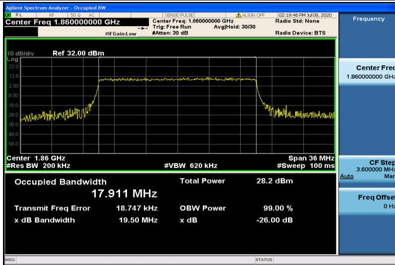
Band2-20MHz-16QAM-18700-100RB#0-17.911
