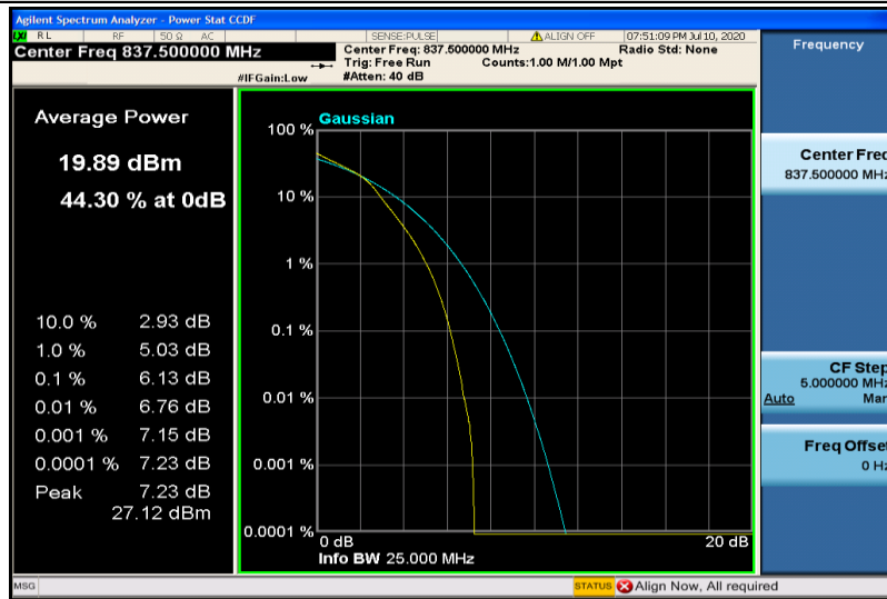
Band19-5MHz-16QAM-24075-25RB#0
