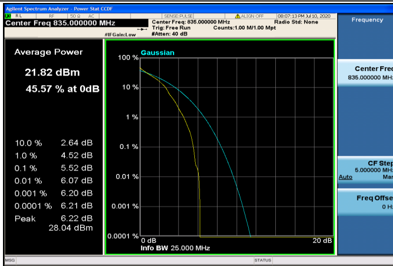
Band19-10MHz-QPSK-24050-1RB#0
