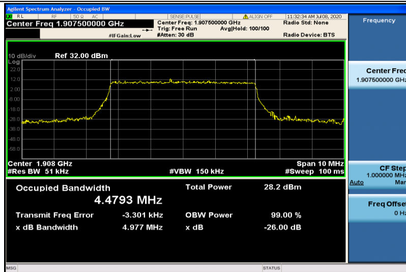
Band2-5MHz-16QAM-19175-25RB#0-4.4793
