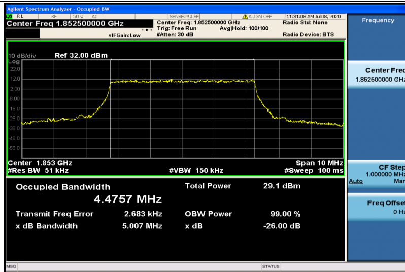
Band2-5MHz-QPSK-18625-25RB#0-4.4757
