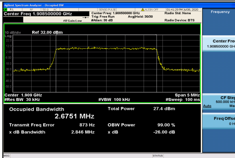
Band2-3MHz-16QAM-19185-15RB#0-2.6751
