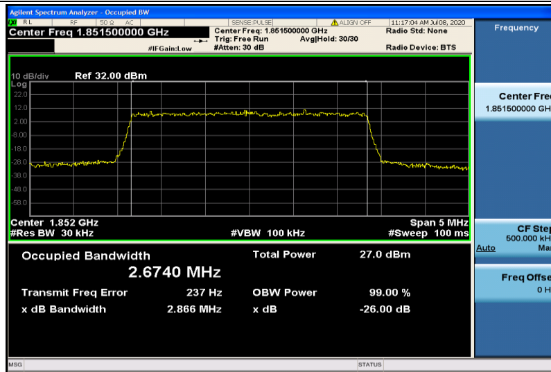
Band2-3MHz-16QAM-18615-15RB#0-2.6740
