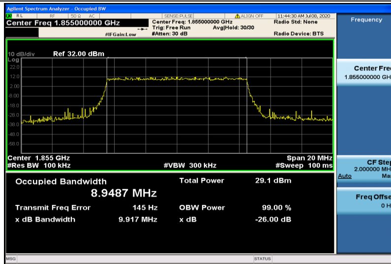
Band2-10MHz-QPSK-18650-50RB#0-8.9487
