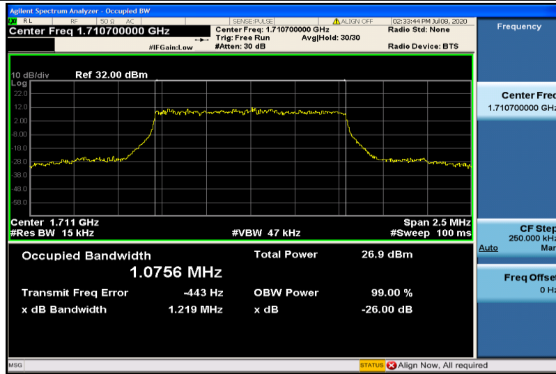
Band4-1.4MHz-16QAM-19957-6RB#0-1.0756
