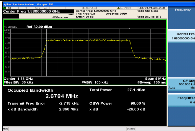
Band2-3MHz-16QAM-18900-15RB#0-2.6784
