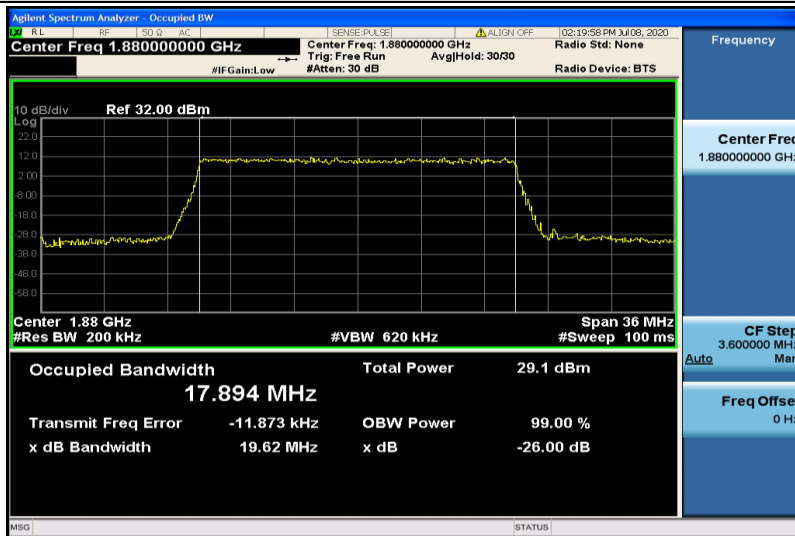
Band2-20MHz-QPSK-18900-100RB#0-17.894
