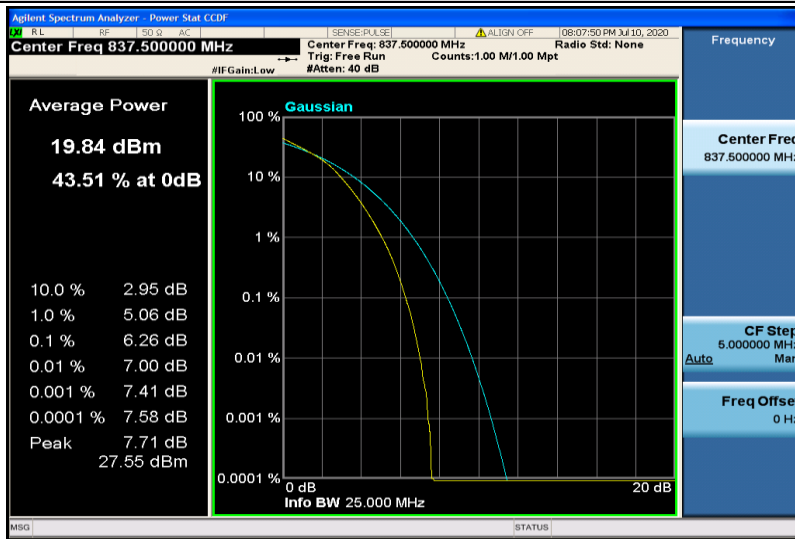
Band19-10MHz-16QAM-24075-50RB#0
