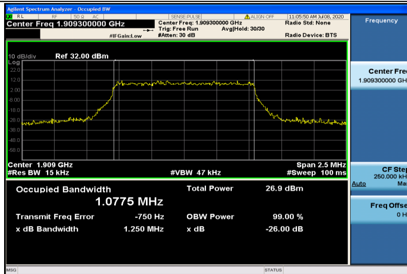
Band2-1.4MHz-16QAM-19193-6RB#0-1.0775
