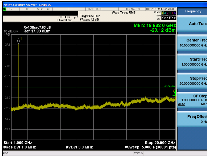
GSM1900-512-1000~20000
