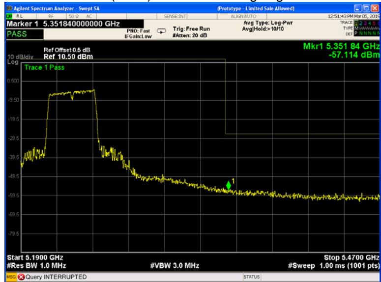
802.11n(HT40) U-NII-1 Band edge-right side
