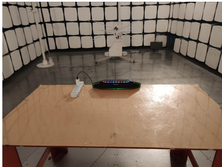
Test Setup for Radiated Emissions(Below 1GHz)
