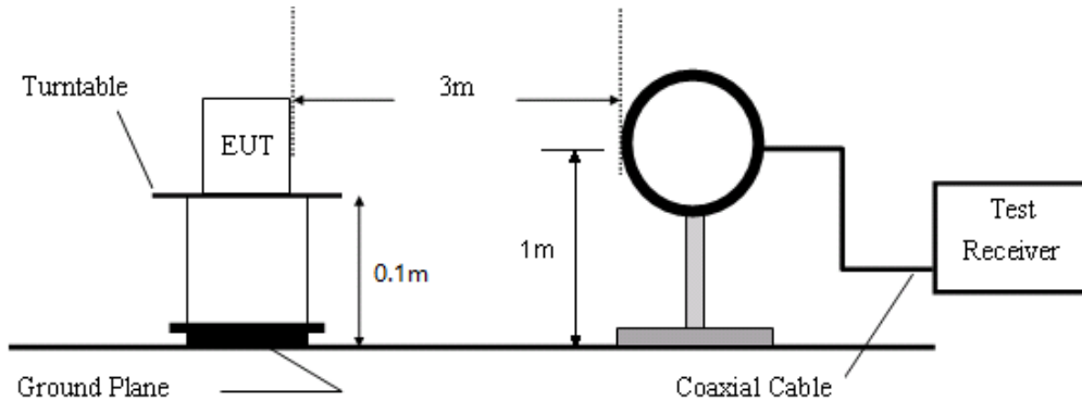
Figure1. Below 30MHz radiated emissions test configuration
