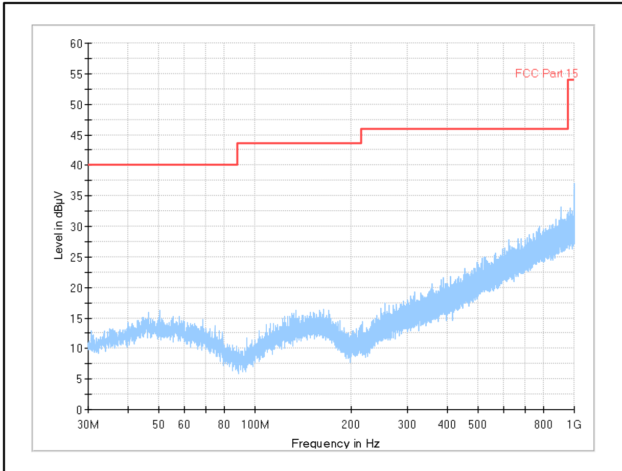
Plot: 30 MHz-1 GHz: Bluetooth Low Energy / Bottom Channel
