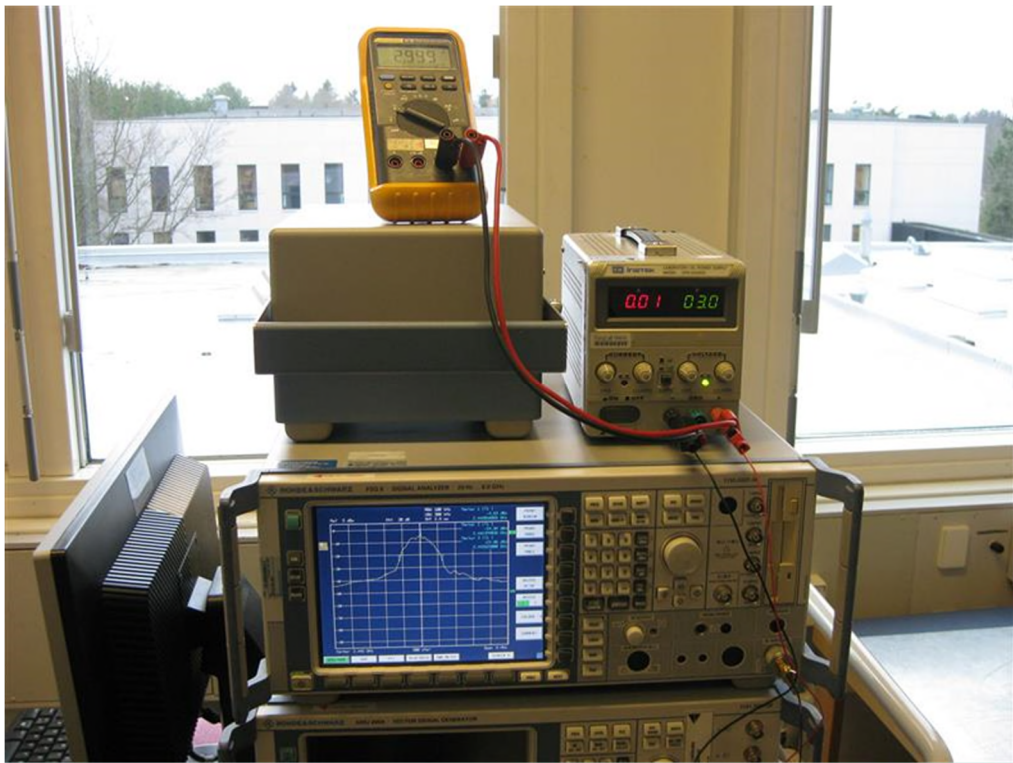
Photo 4.9.1 Test setup regarding measurement of 20 dB bandwidth.
