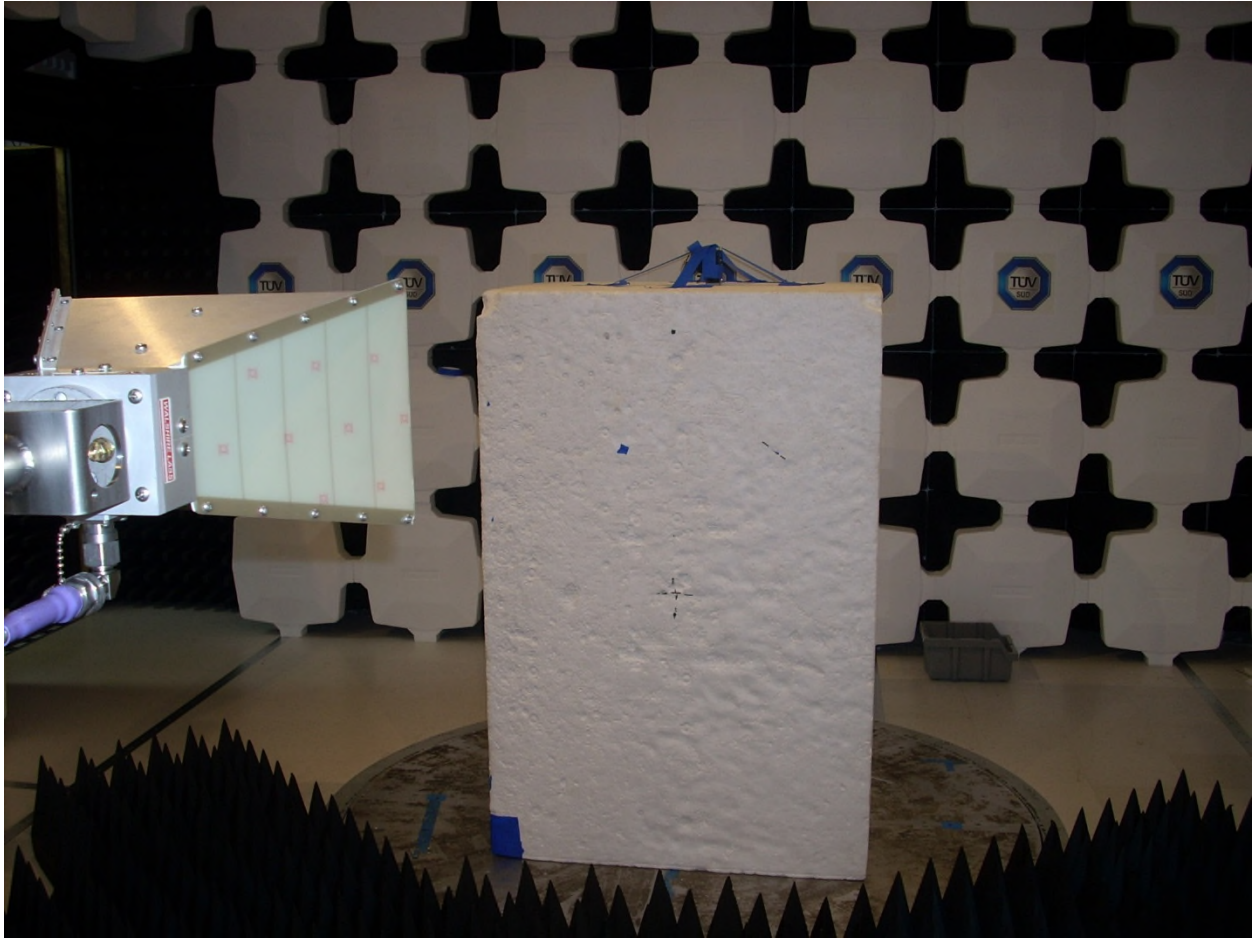
Radiated spurious emissions (1 – 10) GHz Front View
