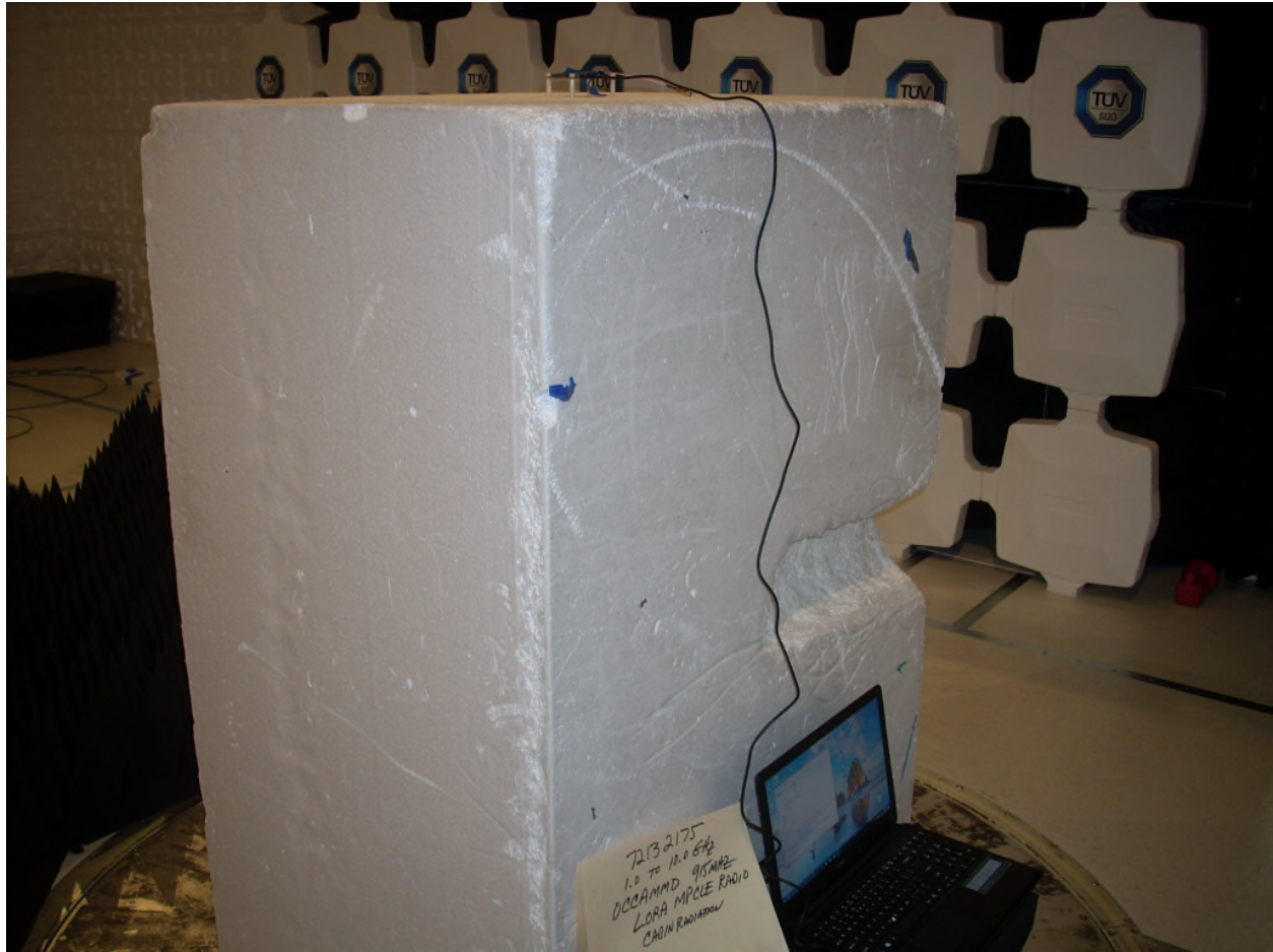
Radiated spurious emissions (1 – 10) GHz Rear View
