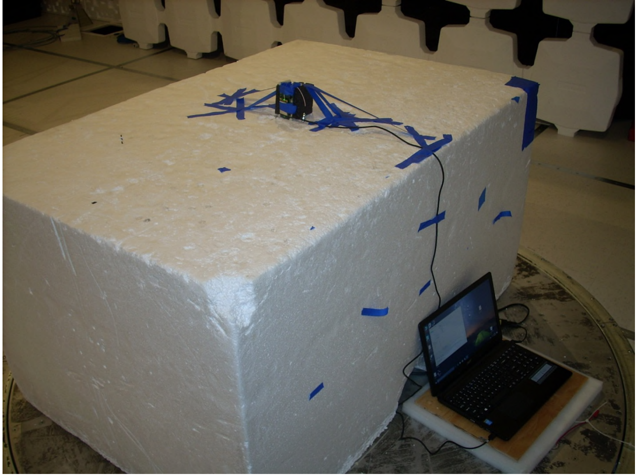
Radiated spurious emissions (30- 1,000) MHz Rear View
