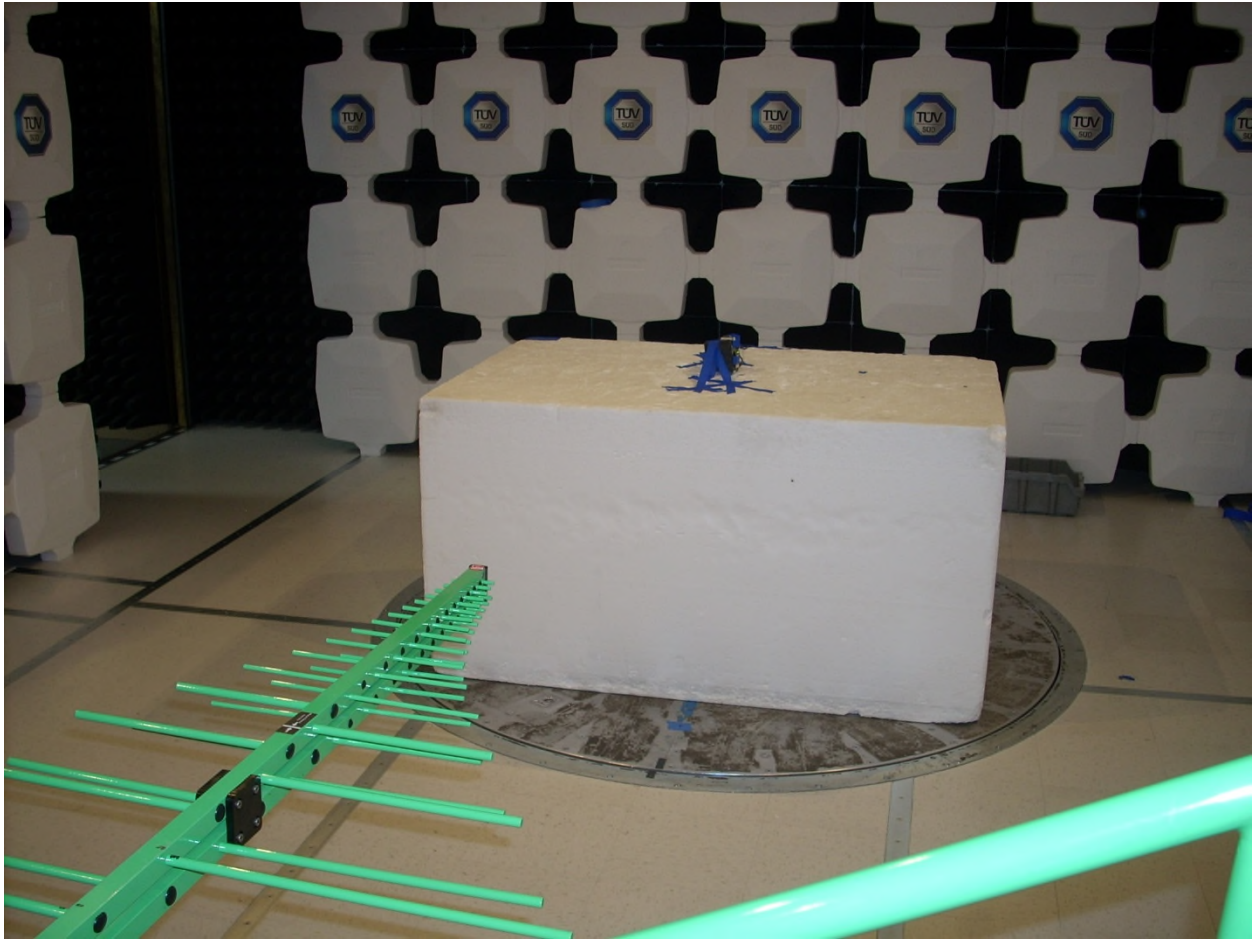
Radiated spurious emissions (30- 1,000) MHz Front View
