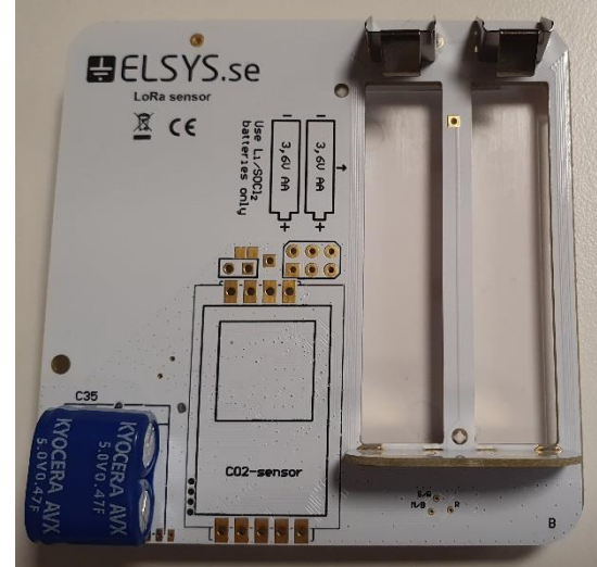
Back-side without CO2 module and batteries Models: ETHd10, ETHdb10, ETHdp10, EVdp10, ESdp10
