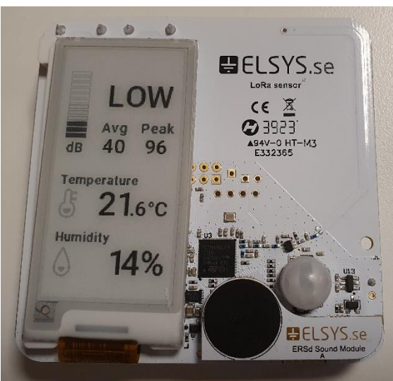
Front-side with PIR. With Sound/VOC-module. Models: EVdp10, ESdp10, EIAQSdp10
