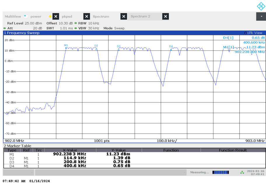
Plot 1: channel separation
