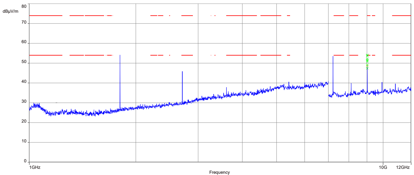
Plot 4: 1 GHz – 12 GHz, horizontal & vertical polarisation (lowest channel) without sound module
