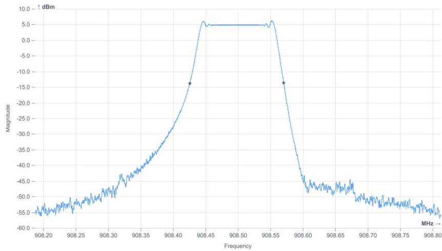
Plot 3: middle channel, 20 dB-BW
