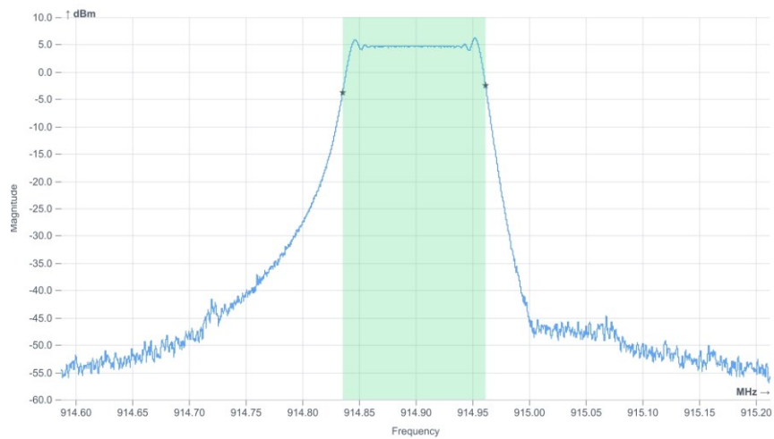
Plot 6: high channel, 99%OBW
