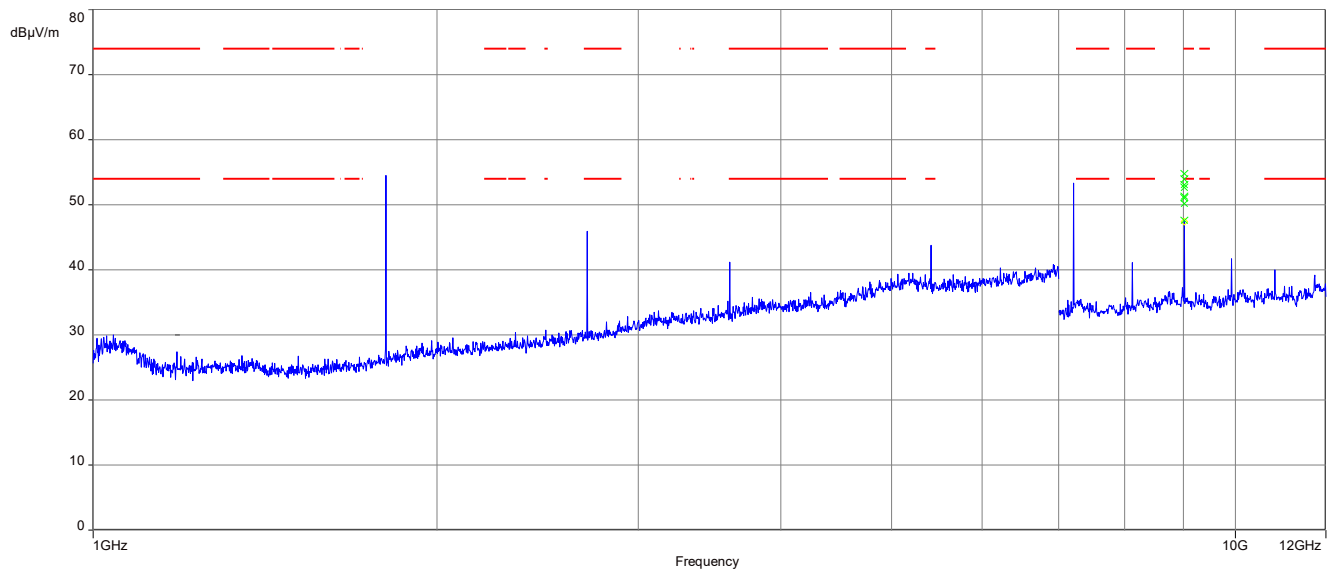
Plot 5: 1 GHz – 12 GHz, horizontal & vertical polarisation (lowest channel) without sound module and CO2 module
