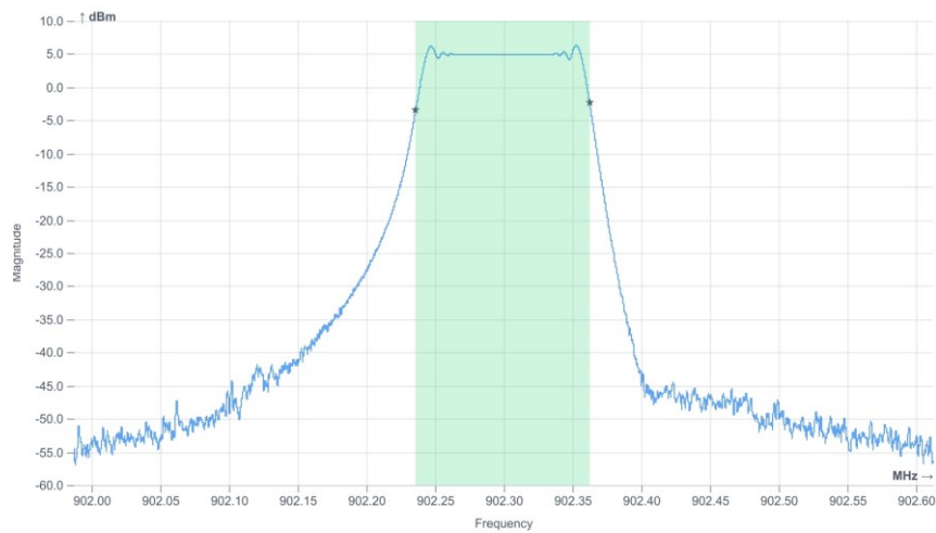
Plot 2: low Channel, 99%OBW
