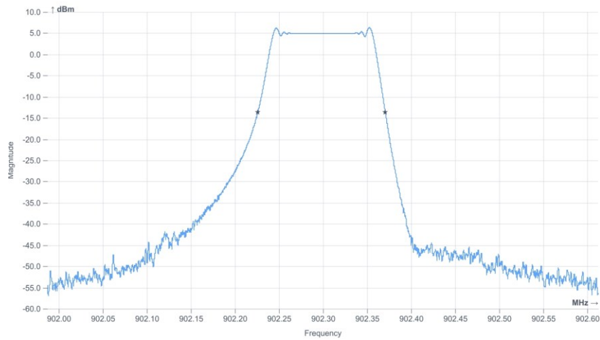
Plot 1: low Channel, 20 dB-BW
