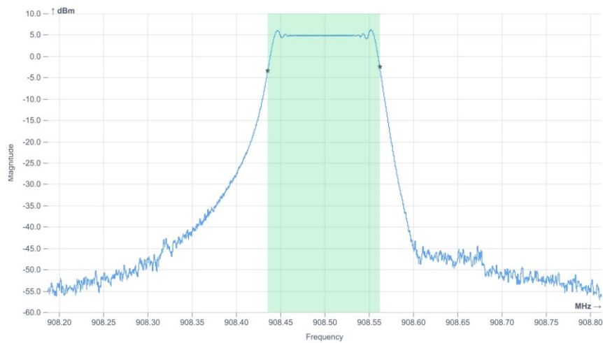
Plot 4: middle channel, 99%OBW
