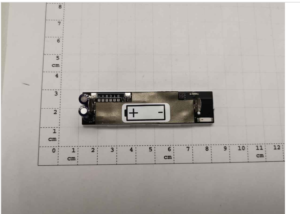
Photograph 4: EUT Inside view (battery removed)
