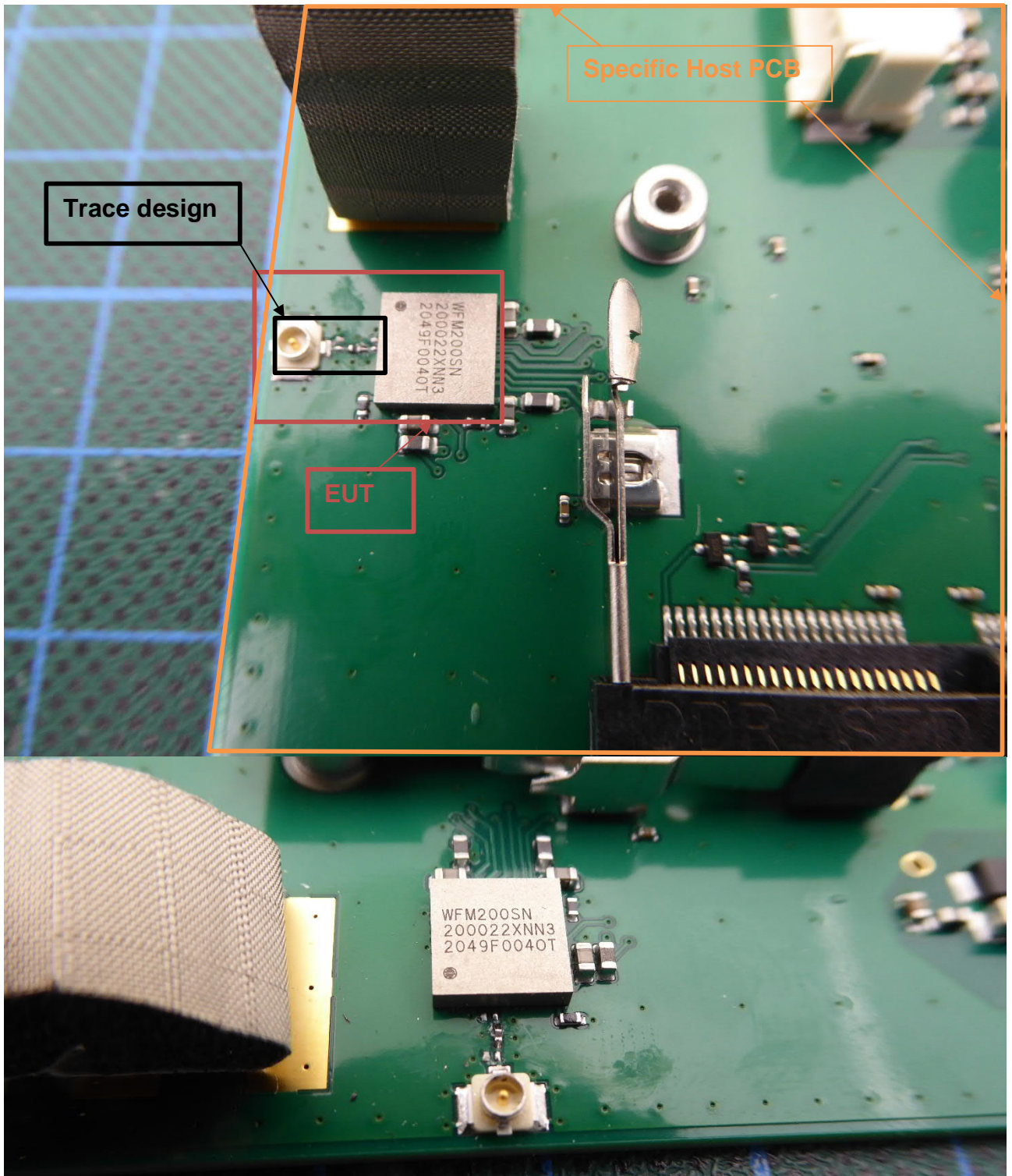
Radio part Detail view
