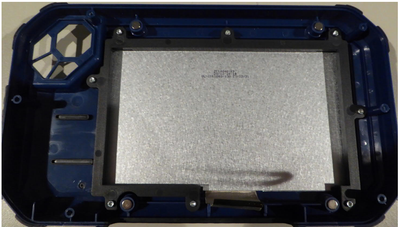
EUT opened Top view
