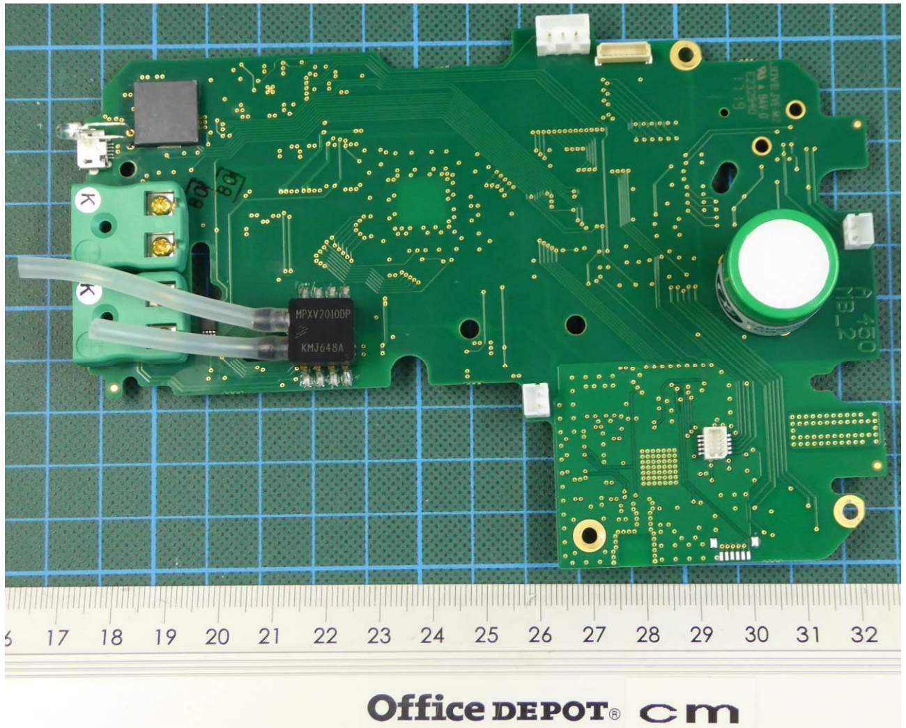
170475eut11.jpg: Main PCB – bottom view
