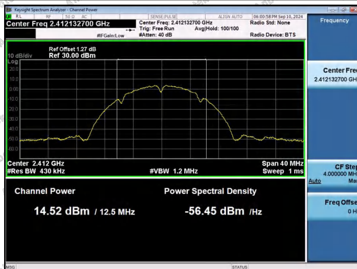
11B-Ant1-2412-PASS
