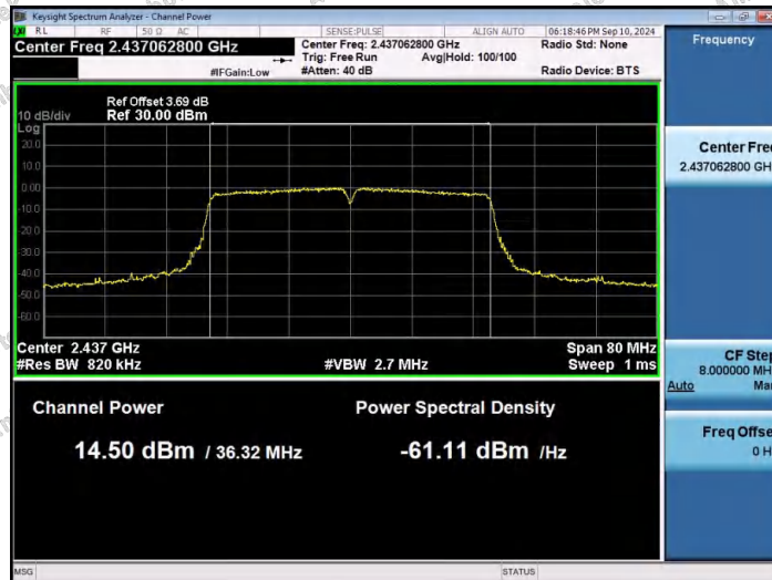
11N40SISO-Ant1-2437-PASS
