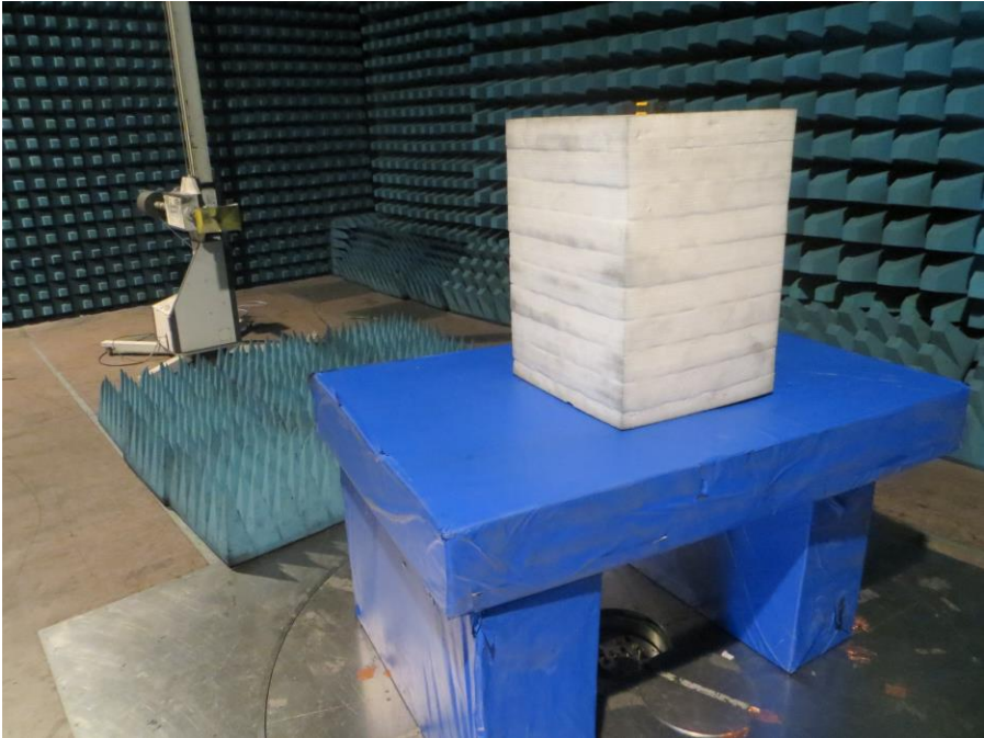
Below 1GHz
