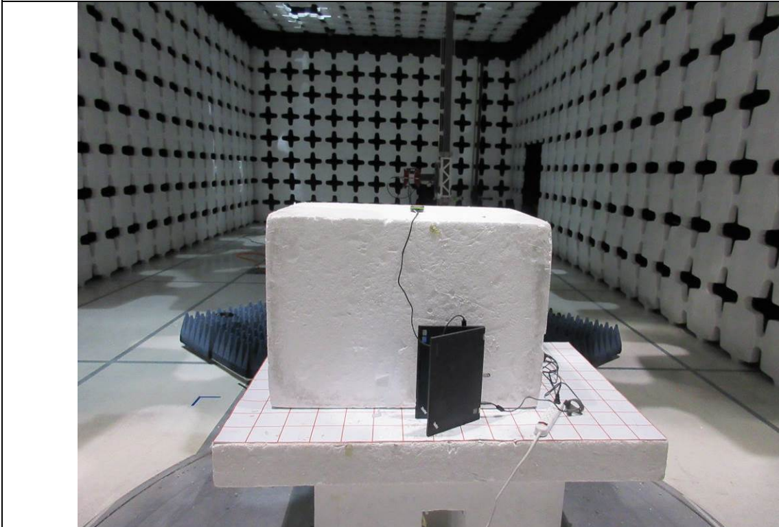
Radiated Emission Test above 1GHz Rear View
