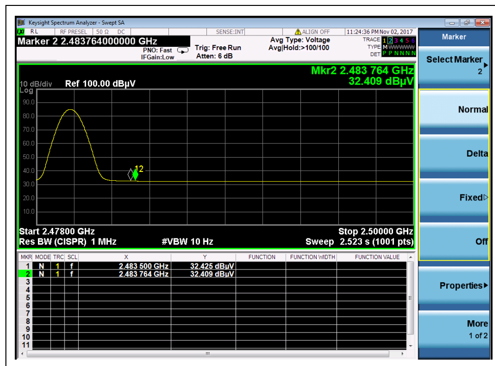
(Plot B2: Channel = 78 AVERAGE @ GFSK)
