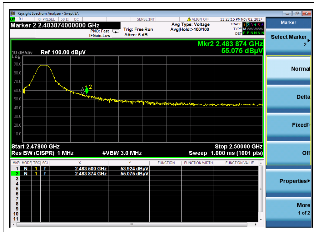
(Plot B1: Channel = 78 PEAK @ GFSK)
