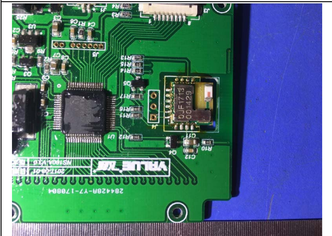
RF Radio Module – Front View
