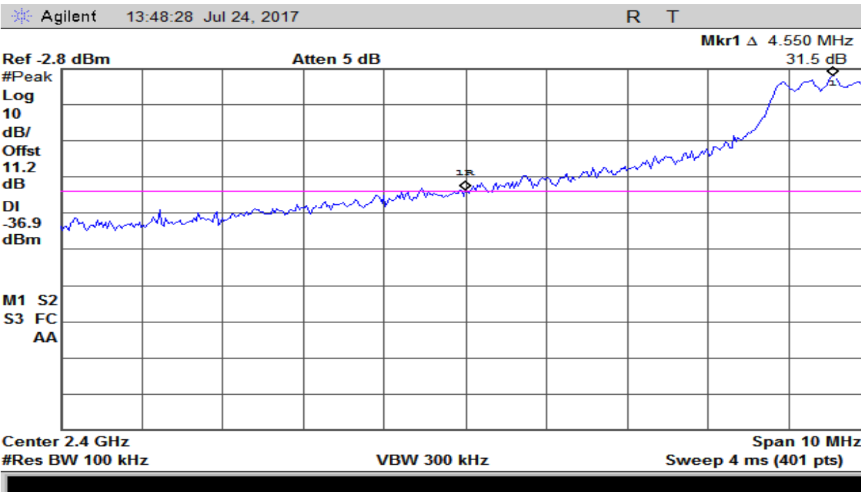
Plot 24 - Band Edge – Low Channel
