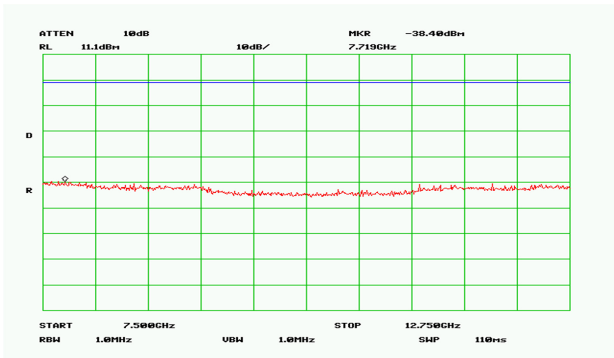
Plot 17 – Mid Band – 7.5GHz to 12.75GHz
