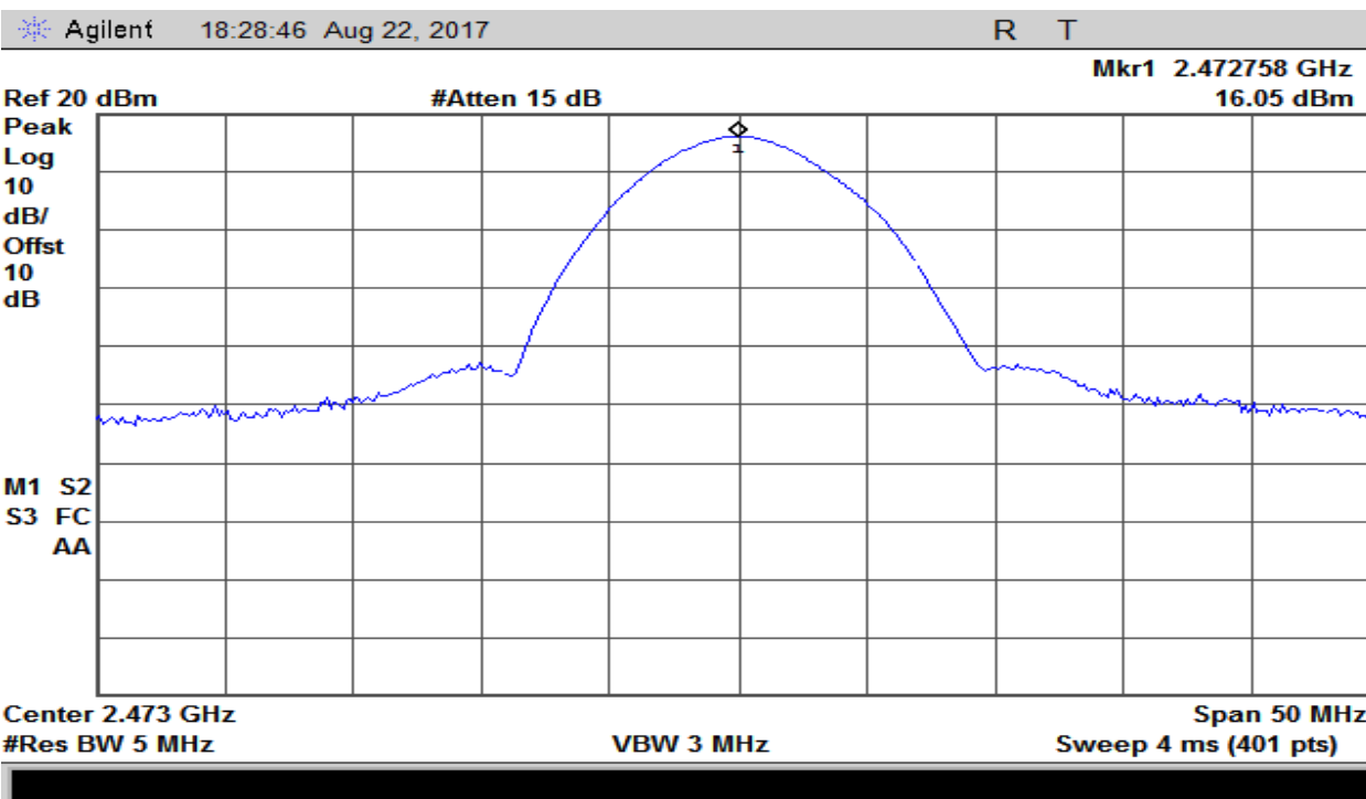
Plot 8 – Output Power – High
