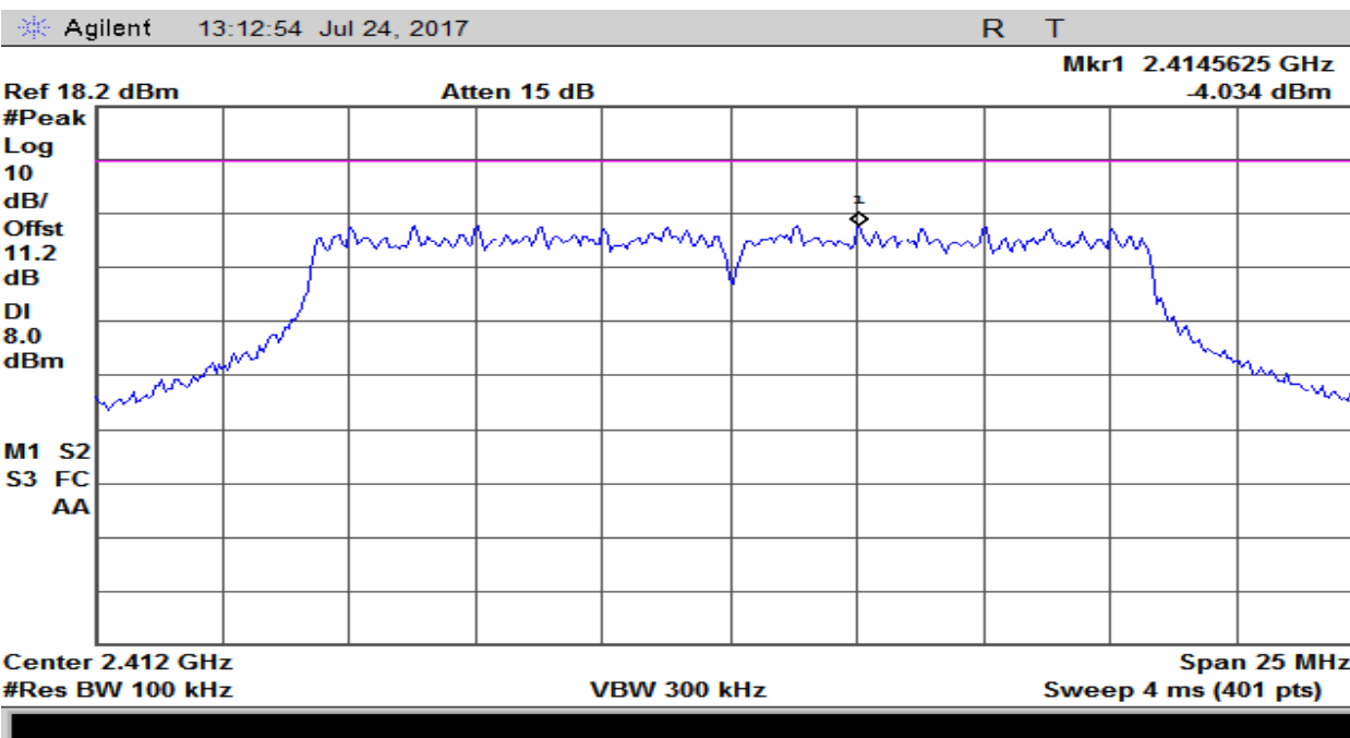
Plot 26 – Power Spectral Density – Lowest Channel
