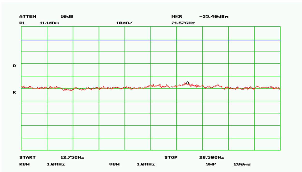
Plot 18 – Mid Band – 12.75GHz to 26.5GHz
