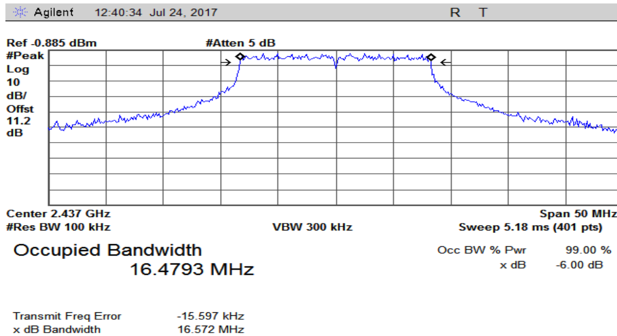
Plot 4 – Middle Channel – 6dB BW
