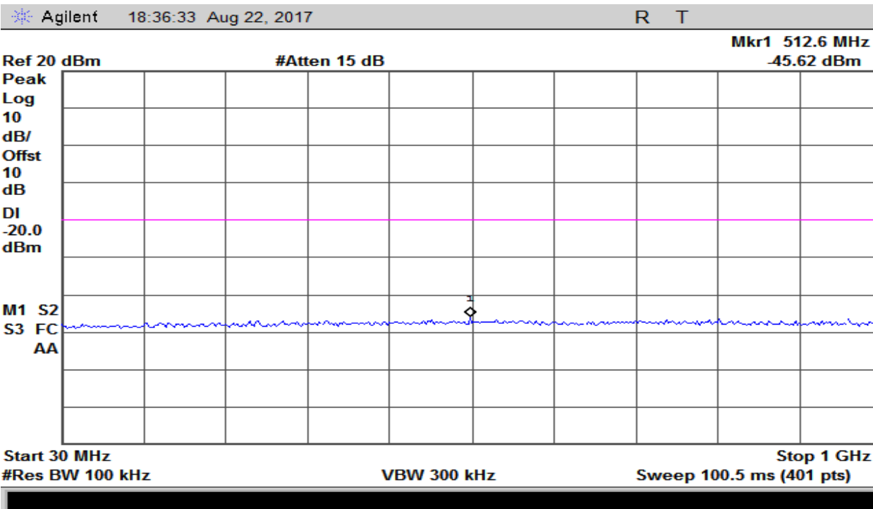
Plot 19 – High Band – 30MHz to 1GHz
