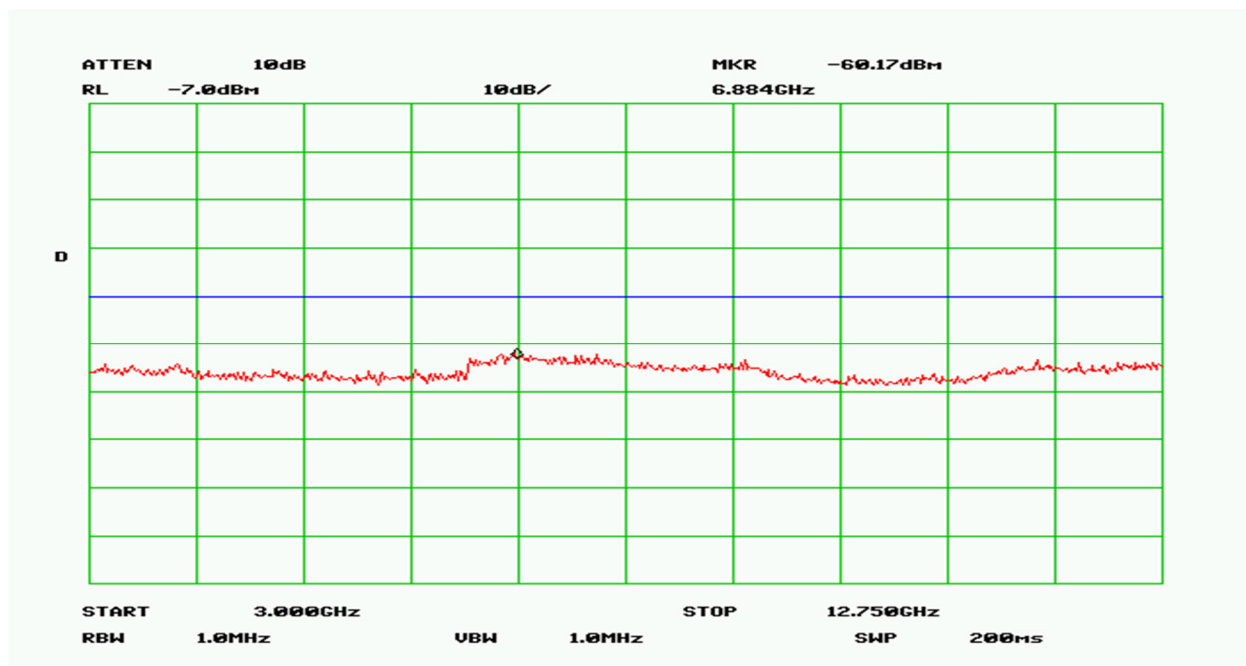
Plot 2 – Receiver Emissions (Conducted) – 1GHz to 12.75 GHz (For Industry Canada RSS-GEN)
