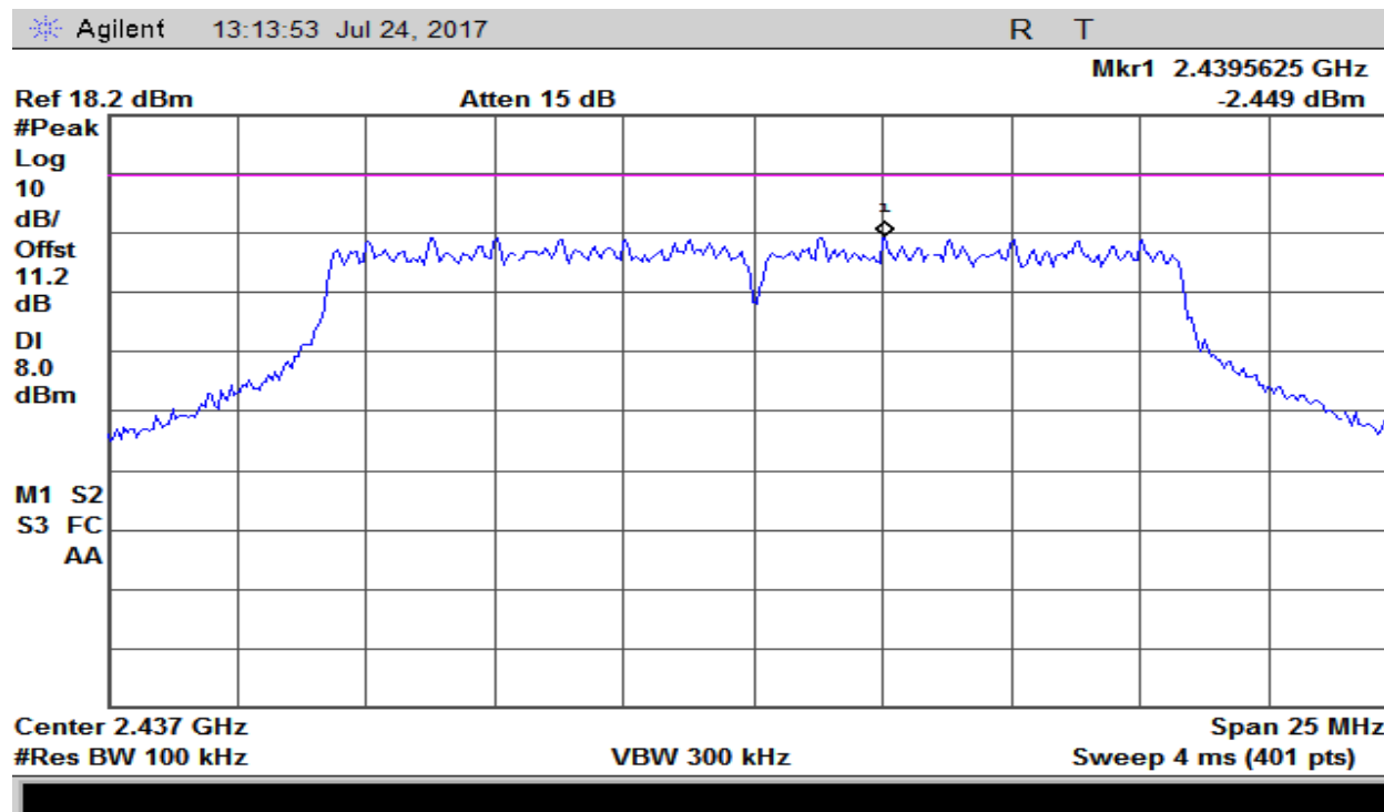
Plot 27 – Power Spectral Density – Middle Channel
