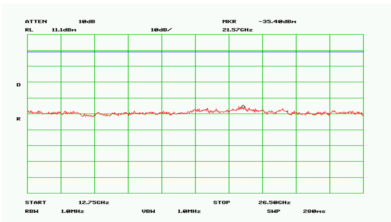
Plot 13 – Low Band – 12.75GHz to 26.5GHz
