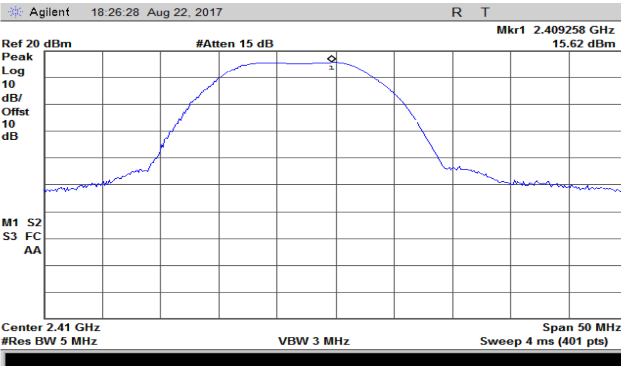
Plot 6 – Output Power – Low
