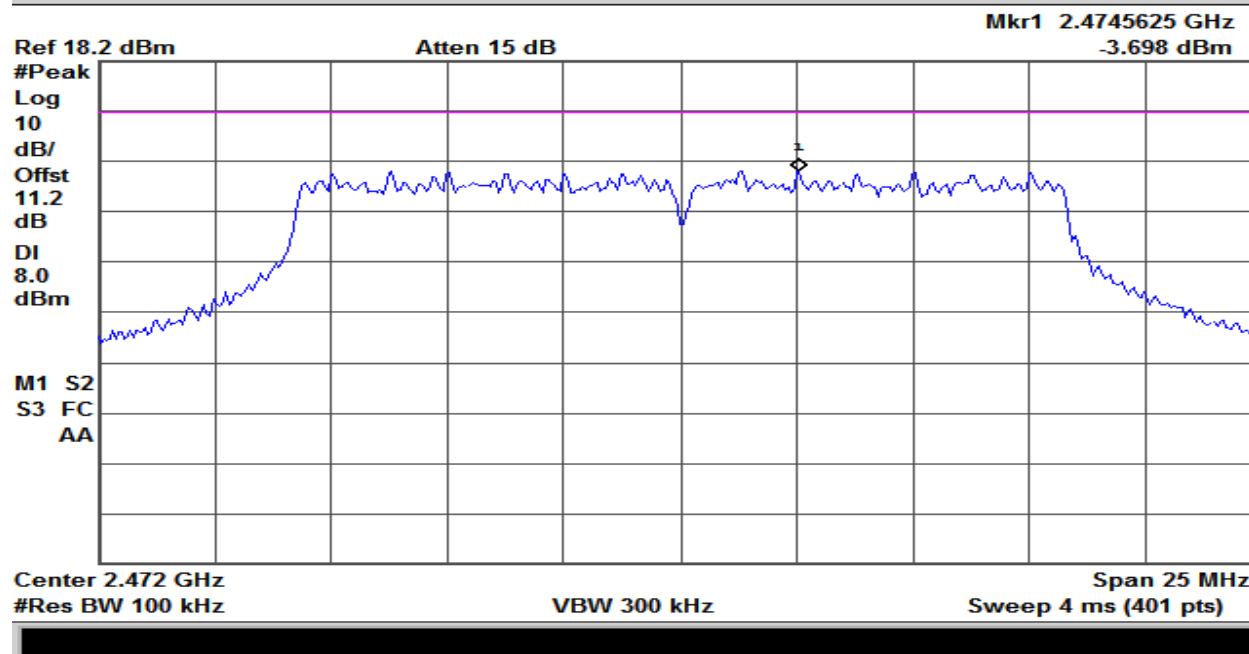
Plot 28 – Power Spectral Density – Highest Channel
