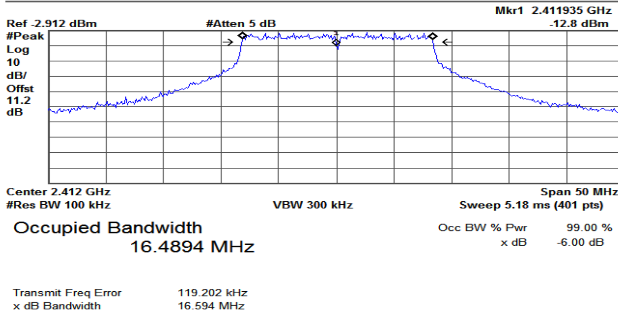
Plot 3 – Lowest Channel – 6dB BW
