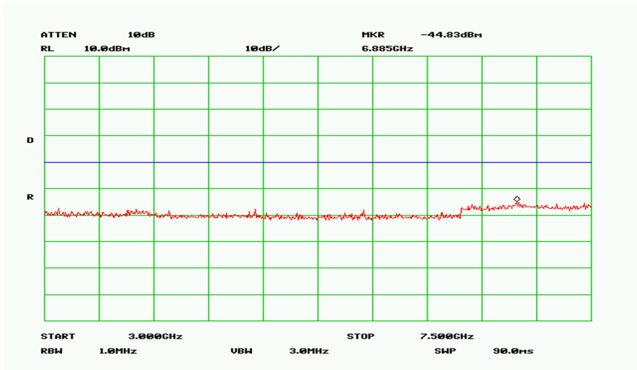
Plot 11 – Low Band – 3GHz to 7.5GHz
