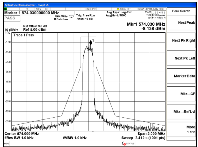
Channel 09 / 574 MHz
