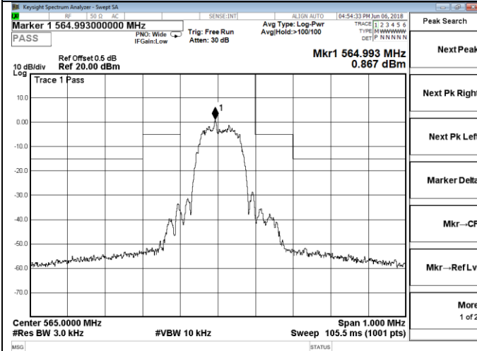
Channel 0 / 565 MHz
