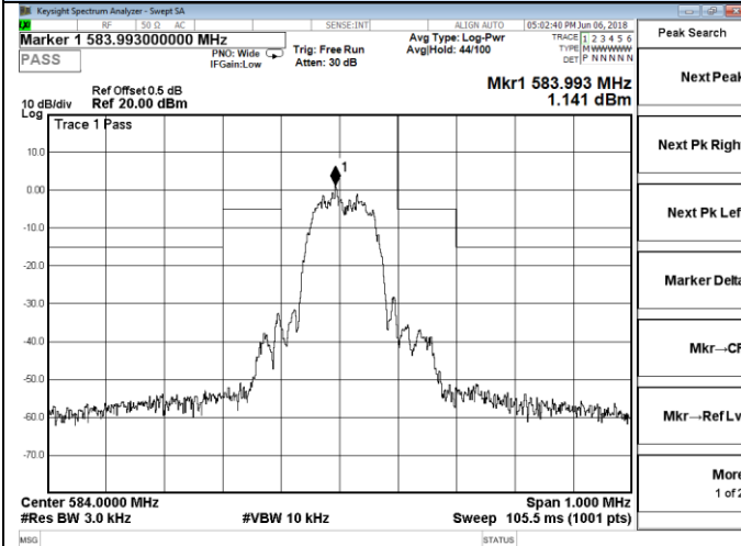
Channel 19 / 584 MHz
