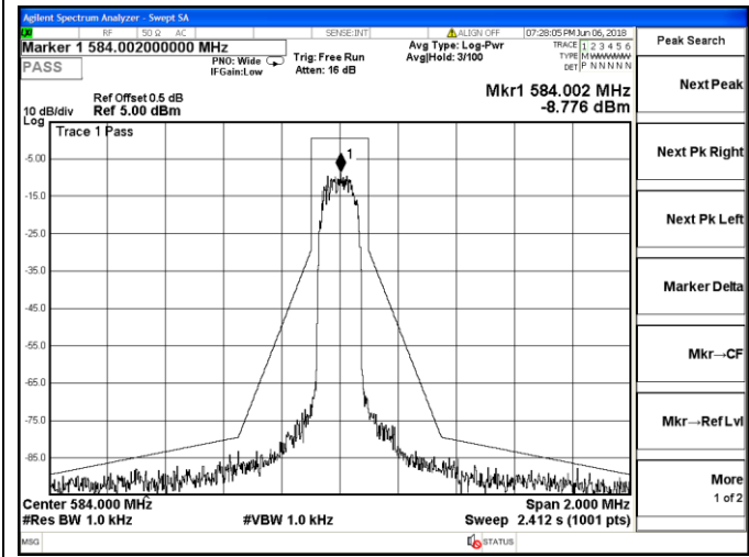
Channel 19 / 584 MHz
