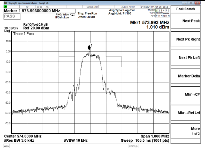
Channel 09 / 574 MHz
