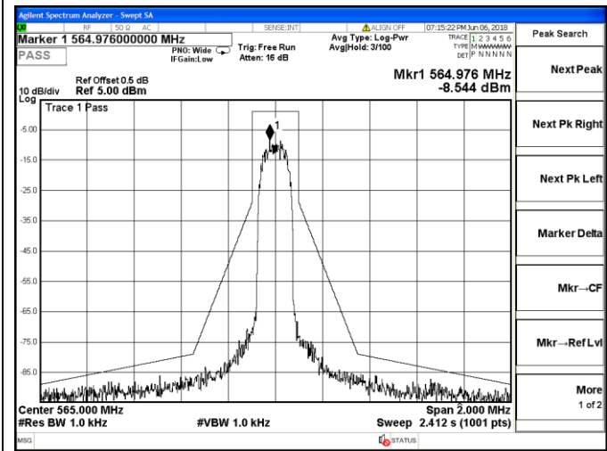
Channel 0 / 565 MHz
