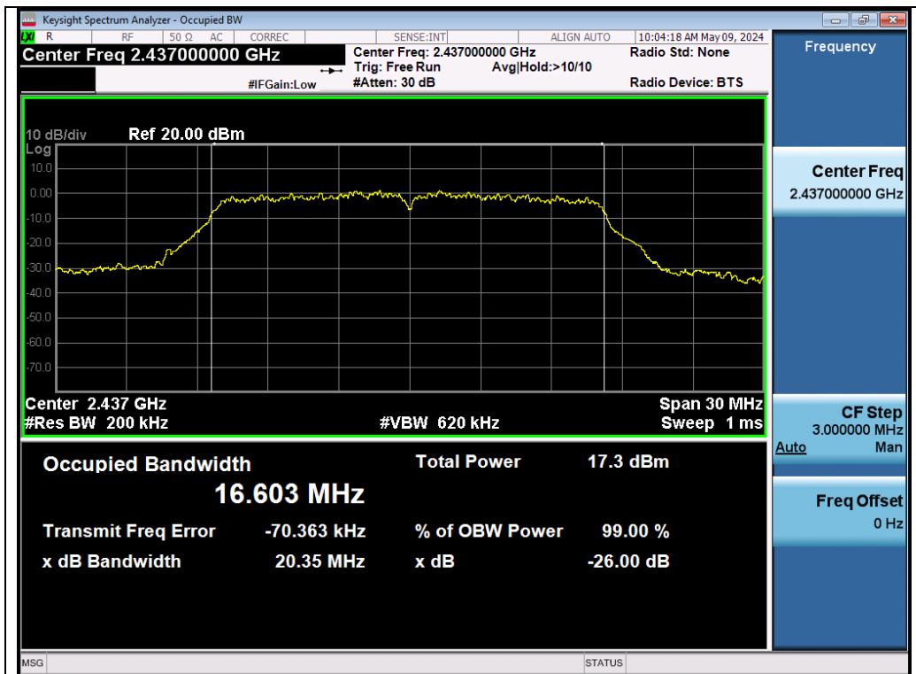
Test_Graph_802.11g_ANT2_2437_6Mbps_OBW
