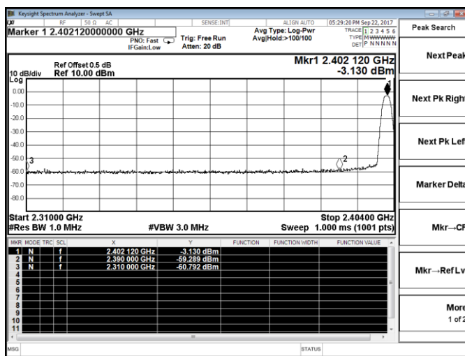
Low Channel / 2402MHz - Peak
