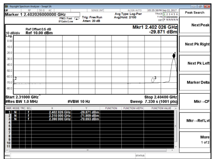
Low Channel / 2402MHz - Average
