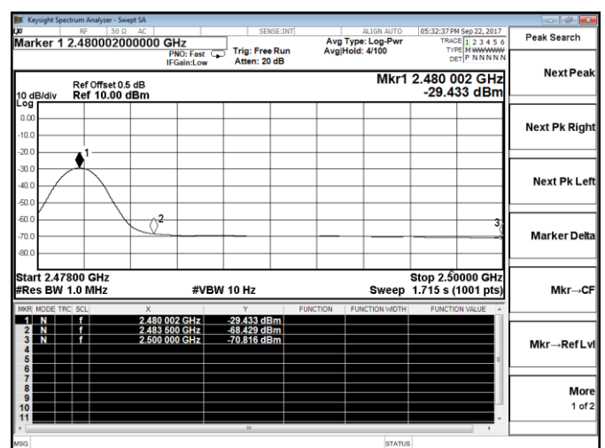
High Channel / 2480MHz - Average
