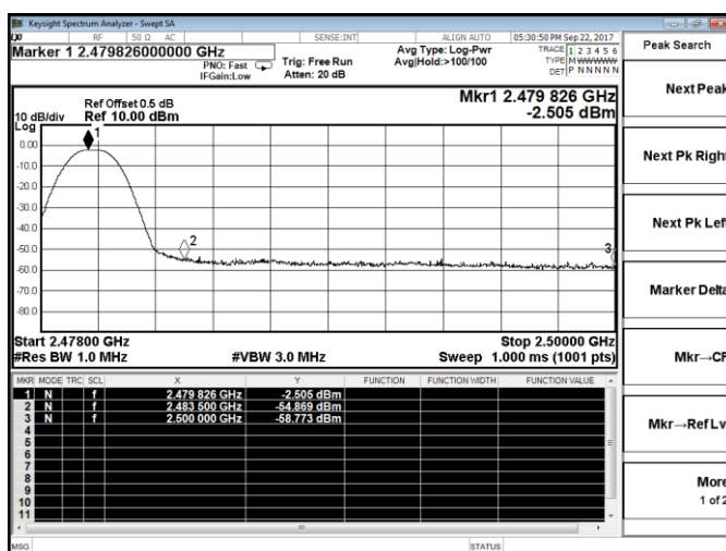
High Channel / 2480MHz - Peak
