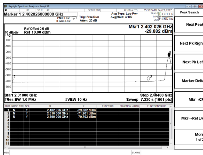
Low Channel / 2402MHz - Average
