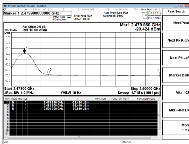
High Channel / 2480MHz - Average
