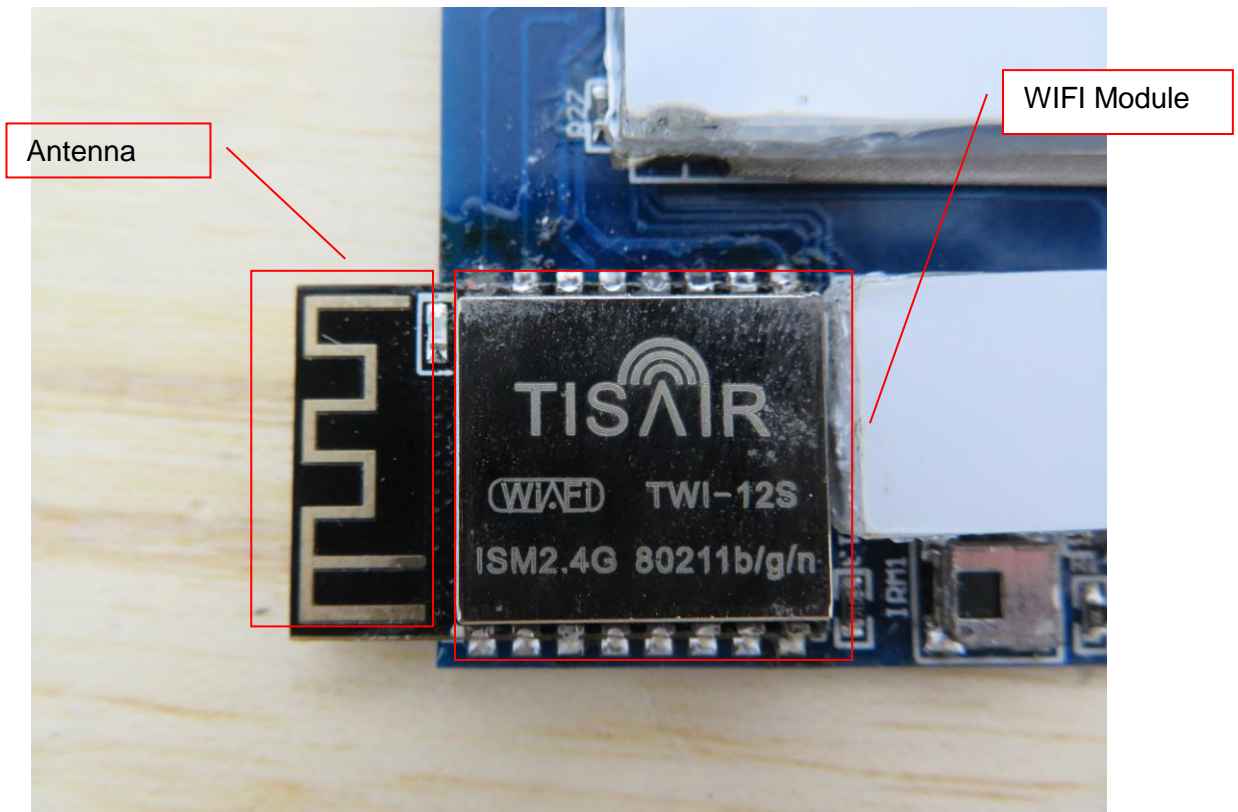
Detail View of Chip
