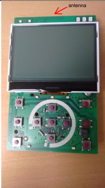
CP with display & wireless - front
