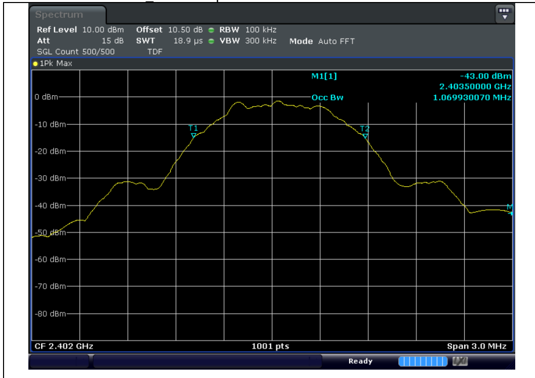
Test mode : 2402 MHz_99% Occupied Bandwidth
