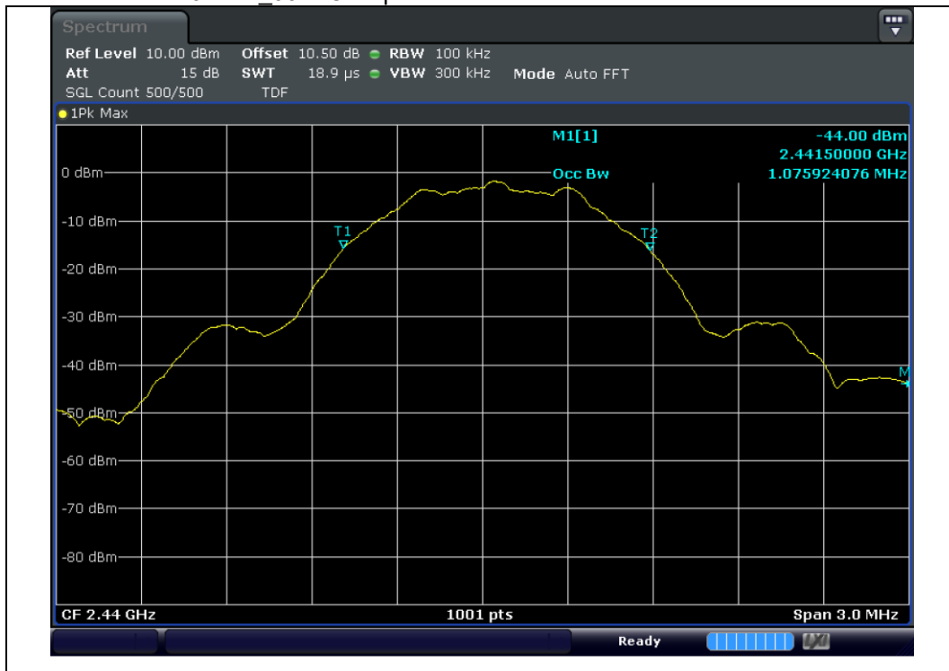
Test mode : 2440 MHz_99% Occupied Bandwidth
