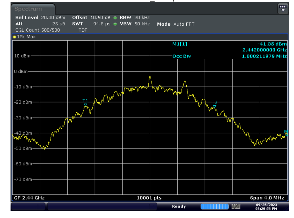
Test mode : Bluetooth LE 2M / 2 440 MHz_Occupied Bandwidth
