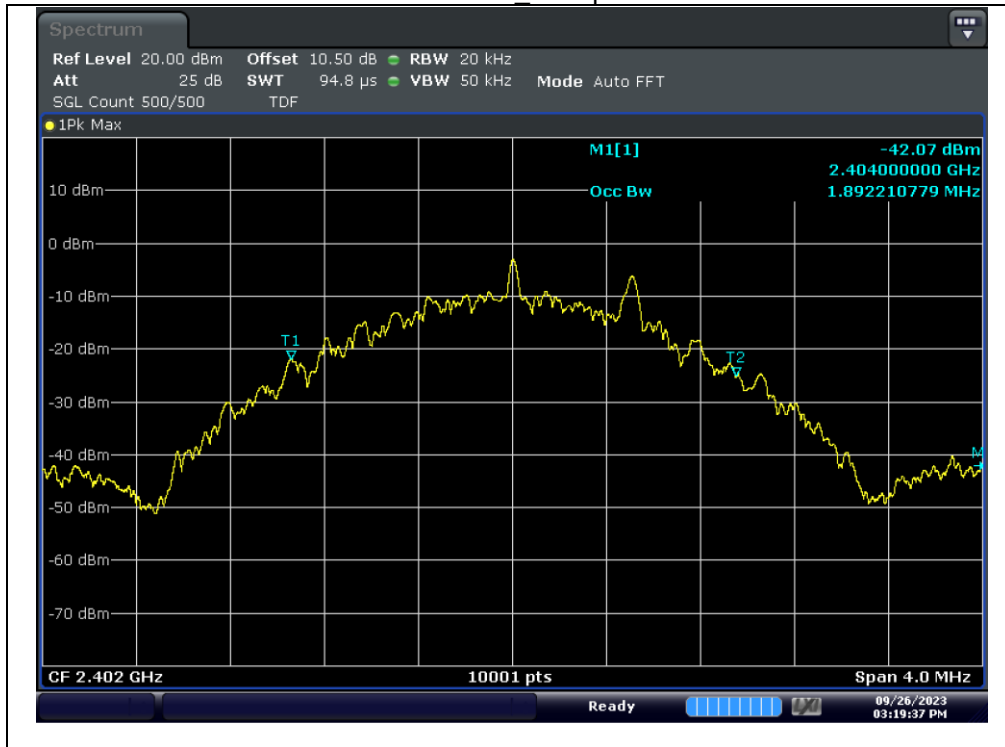
Test mode : Bluetooth LE 2M / 2 402 MHz_Occupied Bandwidth
