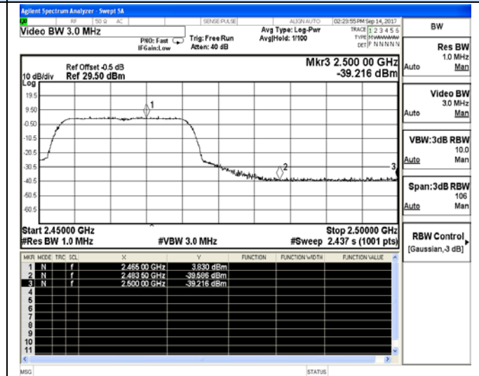
Channel 11 / 2462 MHz – Peak
