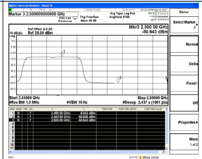
Channel 11 / 2462 MHz – Average
