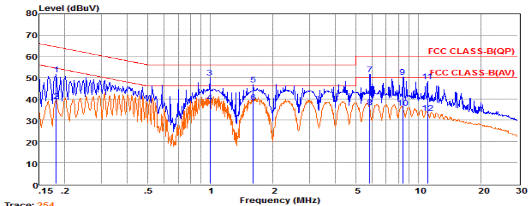
Trace: 254
