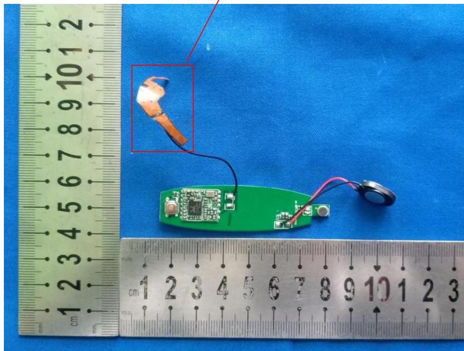
IFA Antenna
