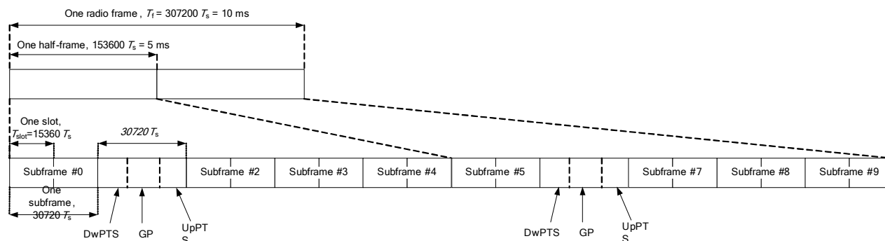
3GPP TS 36.211 Figure 4.2-1: Frame Structure Type 2
