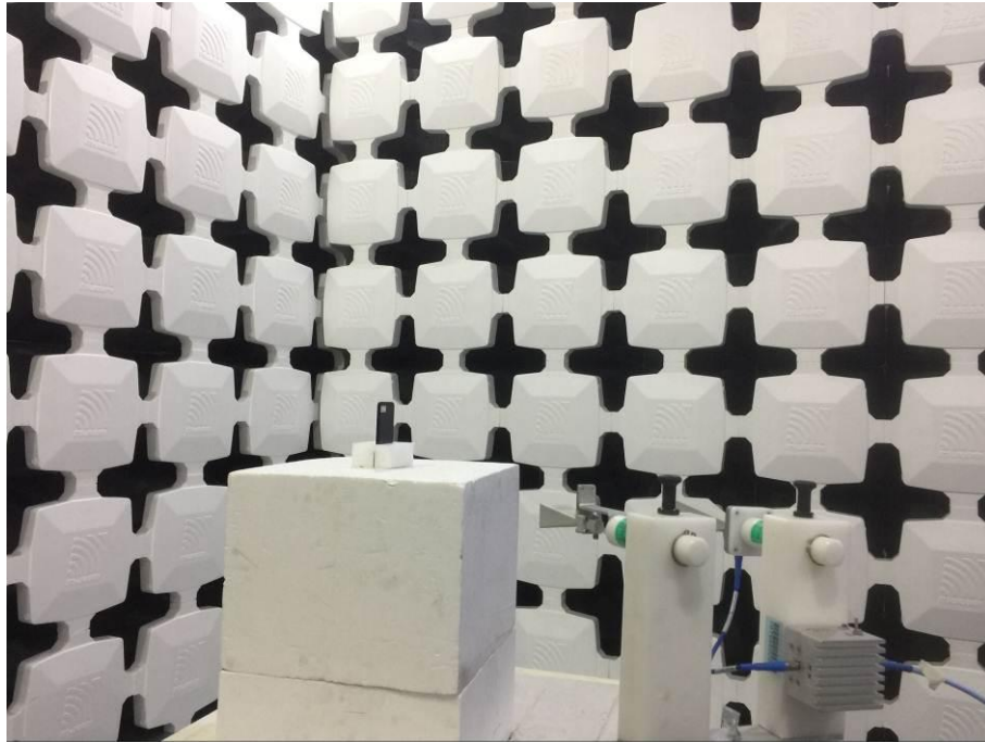
11. Radiated Emissions (Part 22/24) (Above 26.5GHz)
