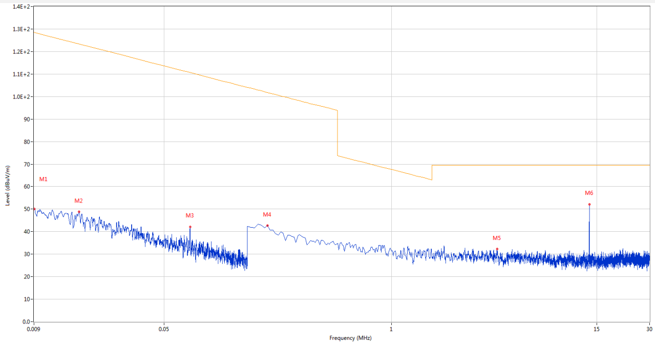
Below 30 MHz, Test Antenna LOOP
