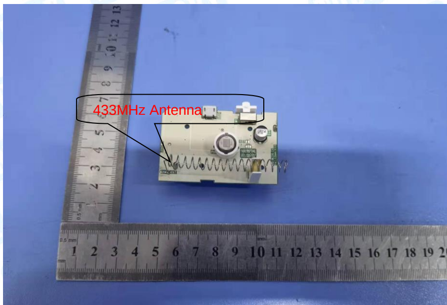
Photo 8 Appearance of PCB
