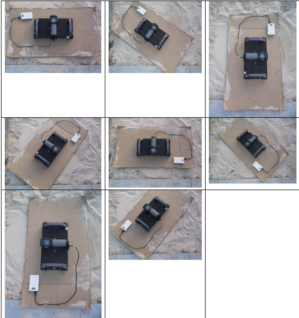
EUT Positions with 45 Degree Interval
