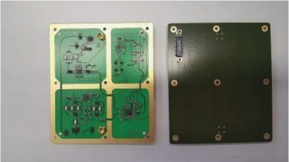
Photo 8: Frontend PCB
