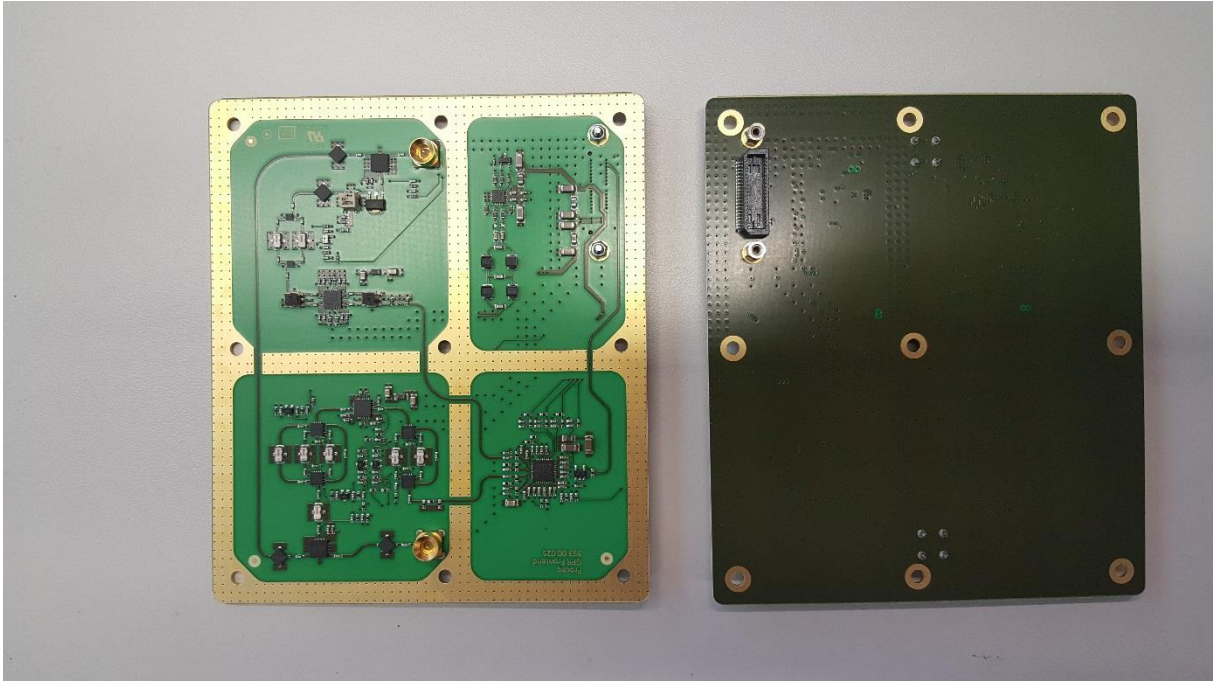
Figure 6: Frontend PCB
