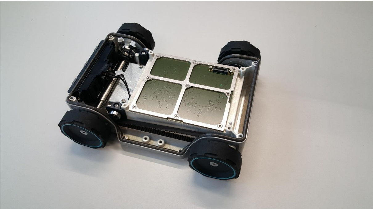
Figure 2: Frontend and Live Wire Detector assembled
