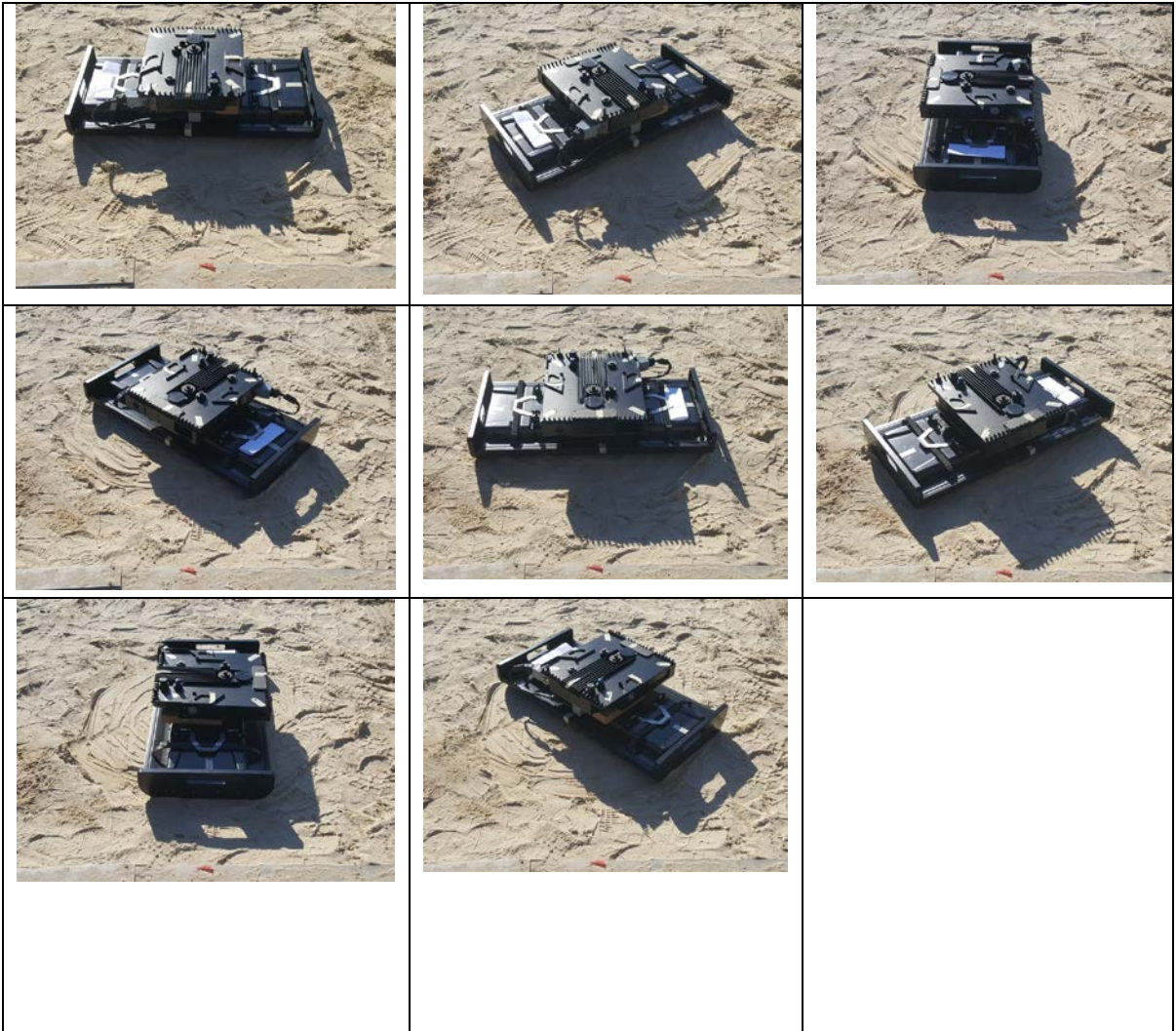
EUT Positions with 45 Degree Interval
