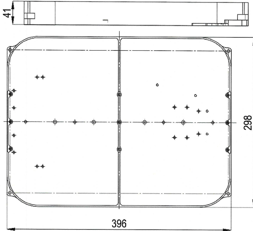
Shielding box
