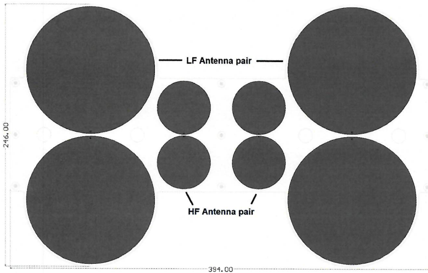
Radiating elements
