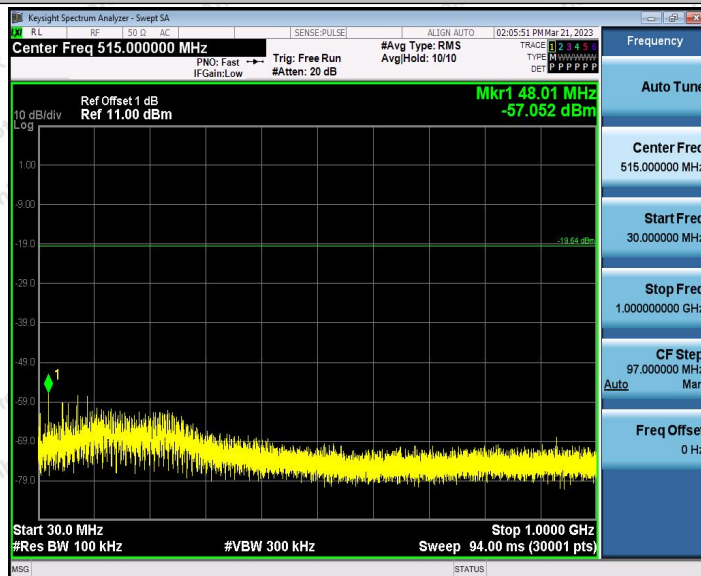
Zigbee_Ant1_2440_30~1000
