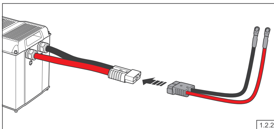
Connect the Anderson Connectors of the batteries to the Adapter Cables (sold separately).
