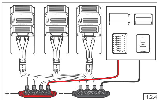
Connect the devices to the Positive and Negative Busbars.
