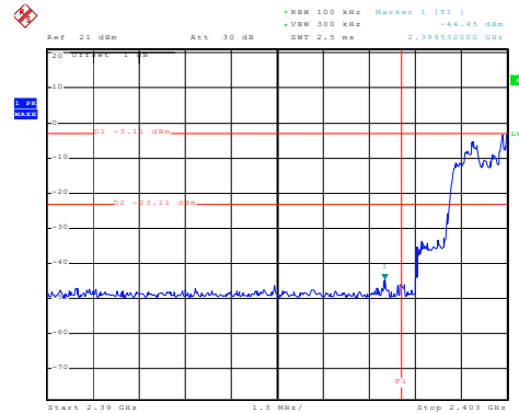
Hopping mode
