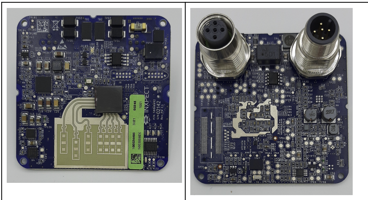
figure 2: top view (on the left) and bottom view (on the right) of the PCB
