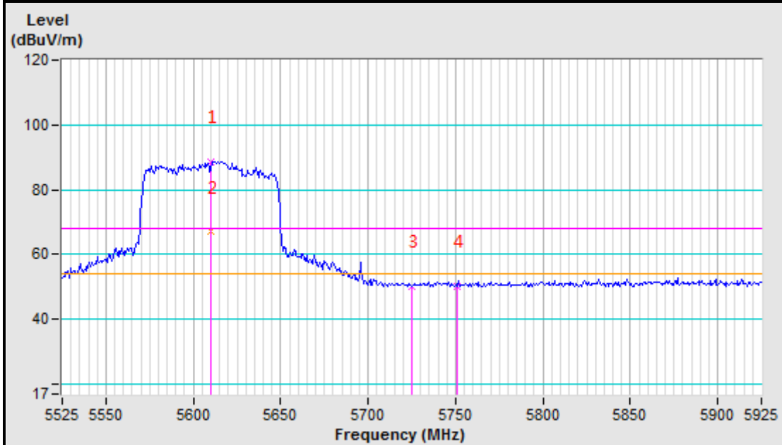
5610MHz Vertical
