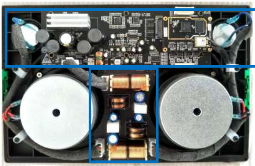
Crossover Board
