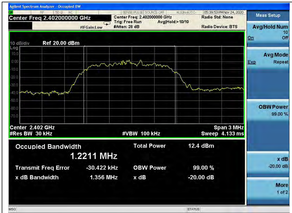
(Channel 0, π/4-DQPSK)
