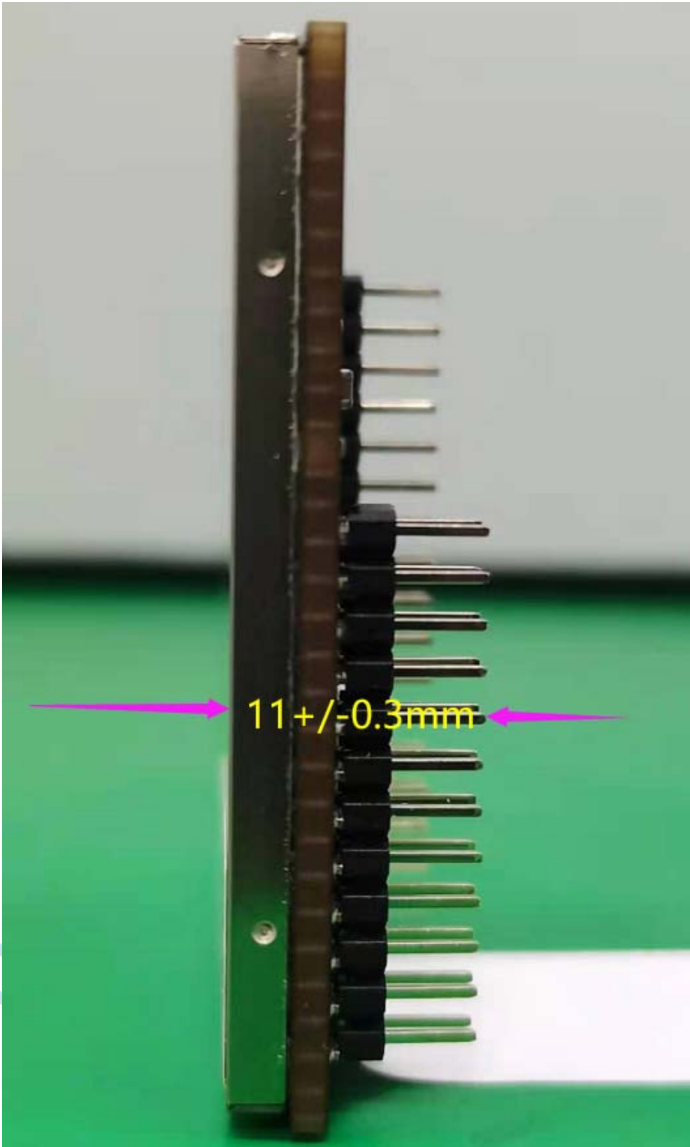
Figure 2- 10 Z dimension
