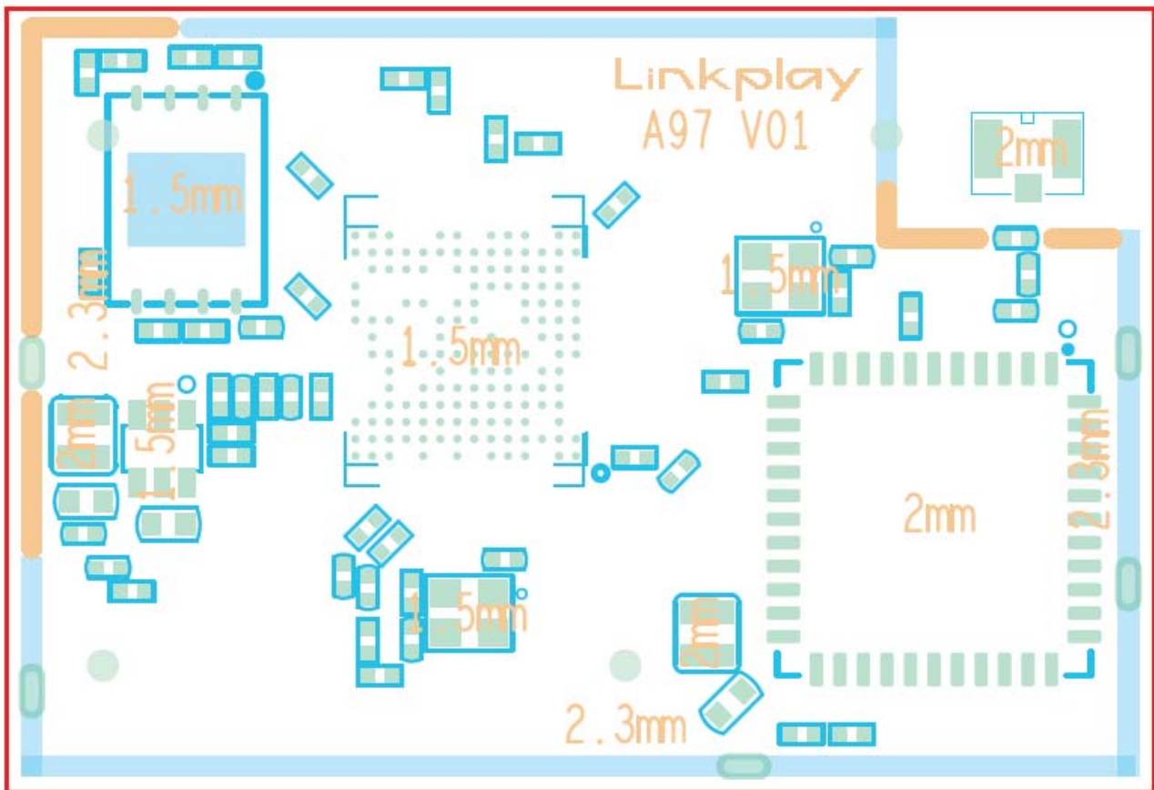
Figure 2-7 Height Limit Top
