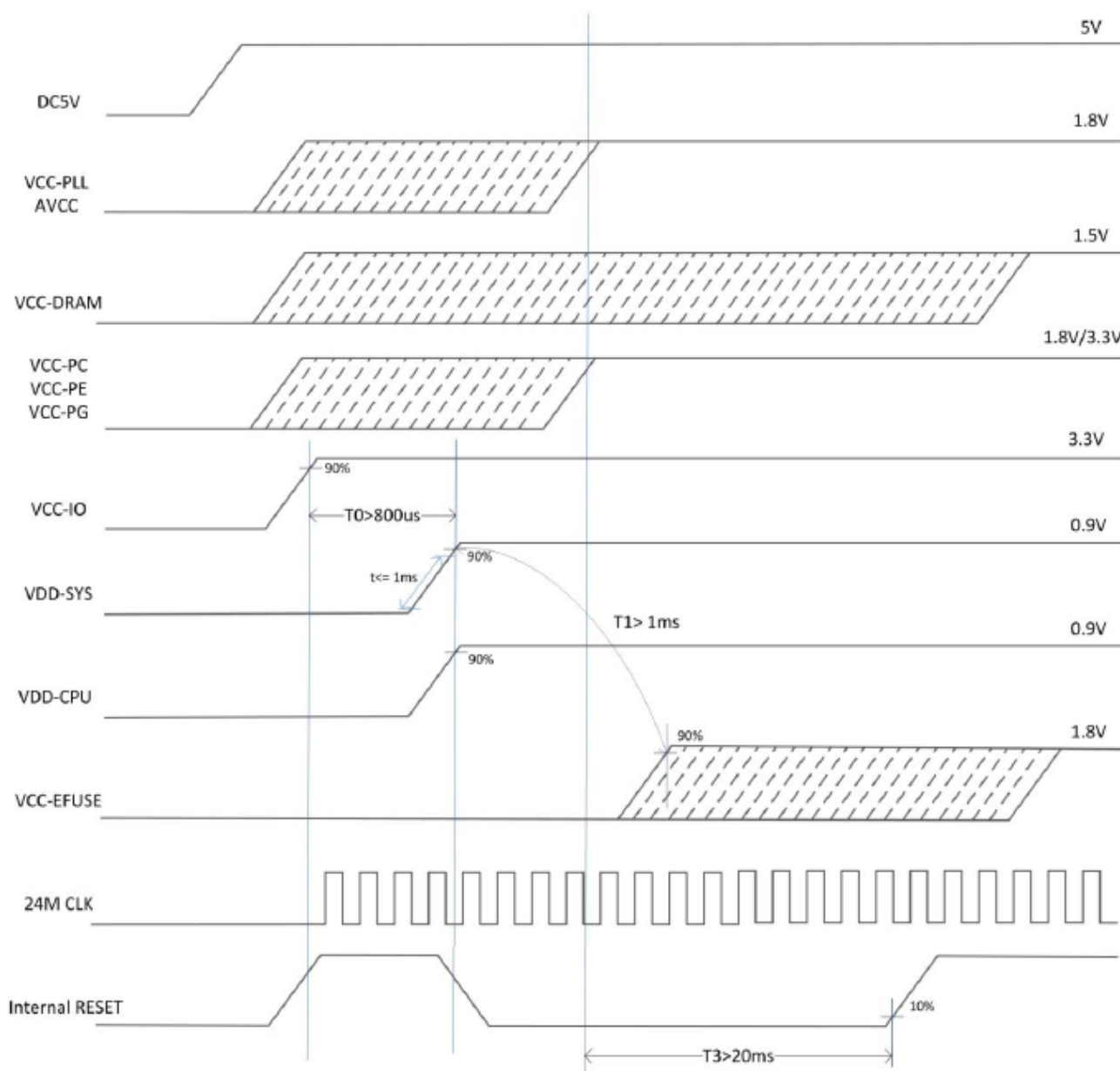
Figure 2- 15 Power on Sequence
