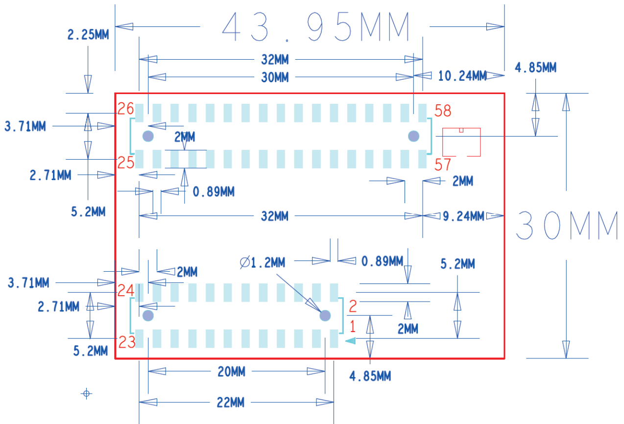
Figure 2-5 A97 Female Socket Dimensions
