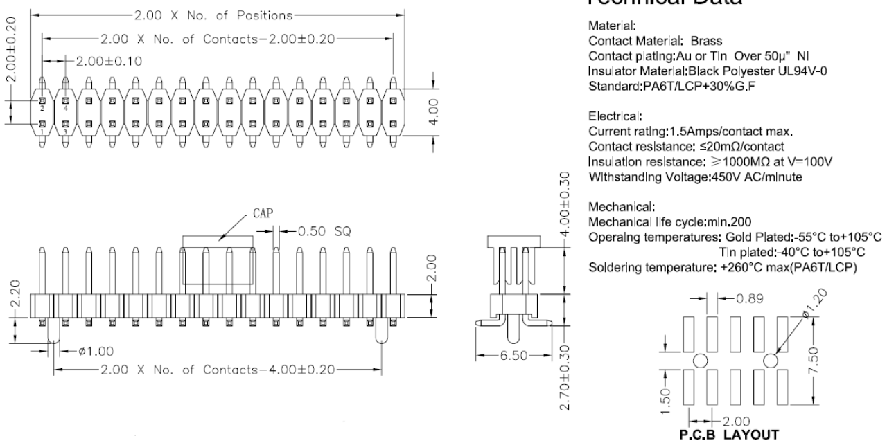
Figure 2-2 Male Pin Header Dimensions
