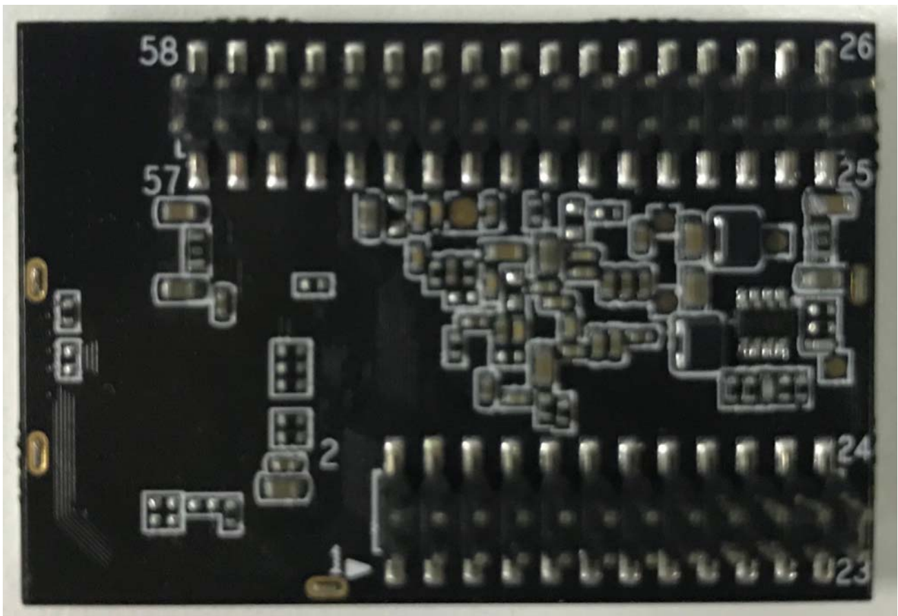
Figure 2-8 Bottom View
