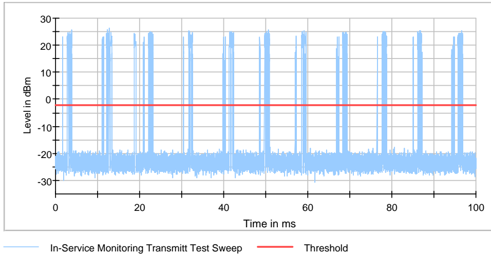
802.11a 5260 MHz_Ant 2
