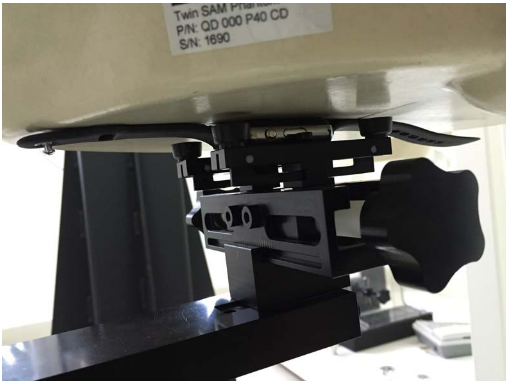
0mm Wrist-worn Setup Photo
