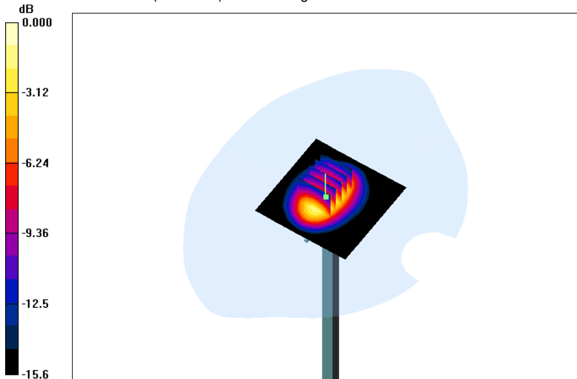
System Performance Check 1900MHz Body 250mW
