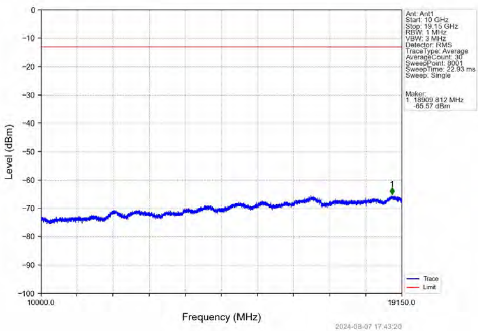
Band25_20MHz_QPSK_MCH_1882.5MHz_RB_1_0_NTNV
