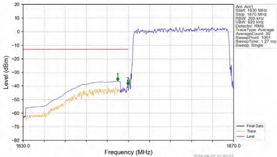
Band25_20MHz_16QAM_LCH_1860MHz_RB_100_0_NTNV
