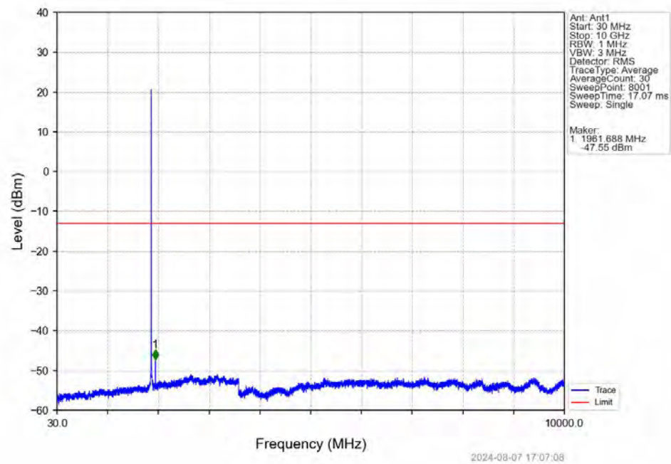
Band25_3MHz_QPSK_MCH_1882.5MHz_RB_1_0_NTNV
