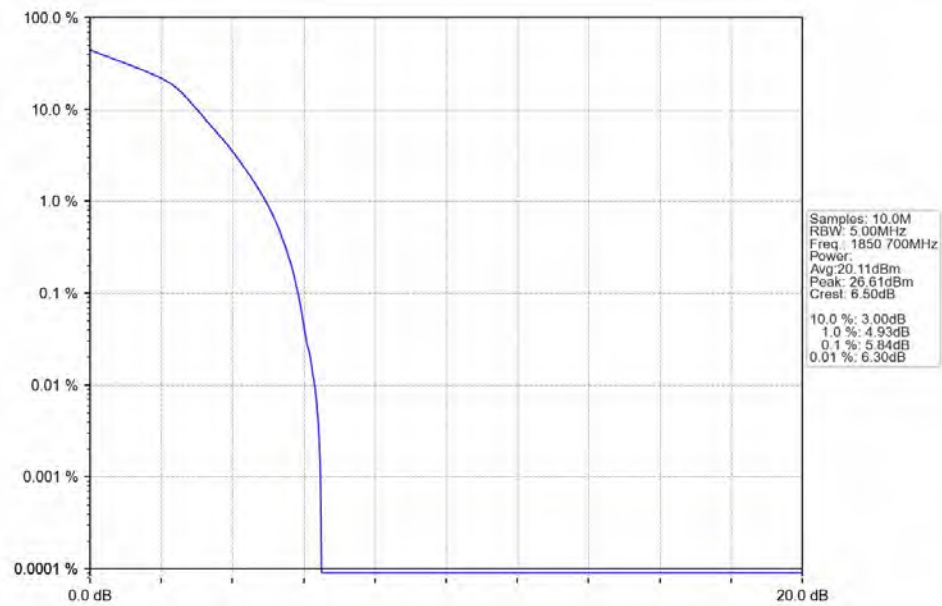
Band25_1.4MHz_16QAM_LCH_1850.7MHz_RB_6_0_NTNV
