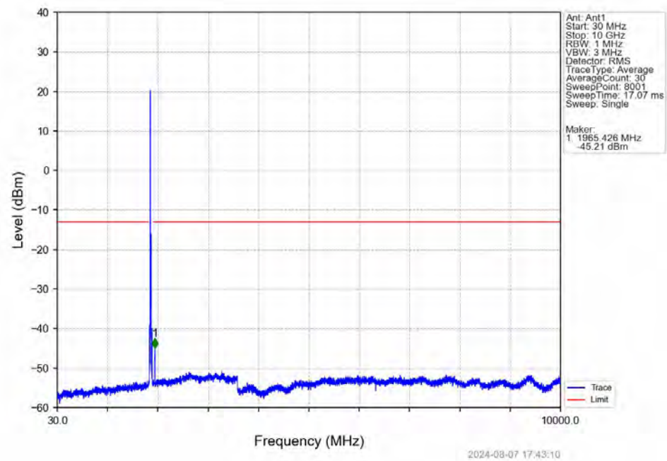
Band25_20MHz_QPSK_MCH_1882.5MHz_RB_1_0_NTNV
