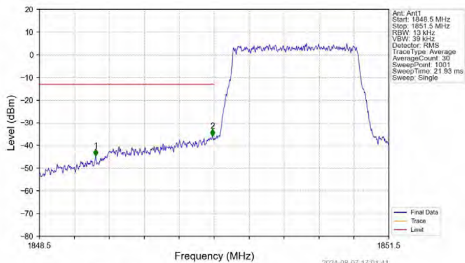
Band25_1.4MHz_QPSK_LCH_1850.7MHz_RB_6_0_NTNV
