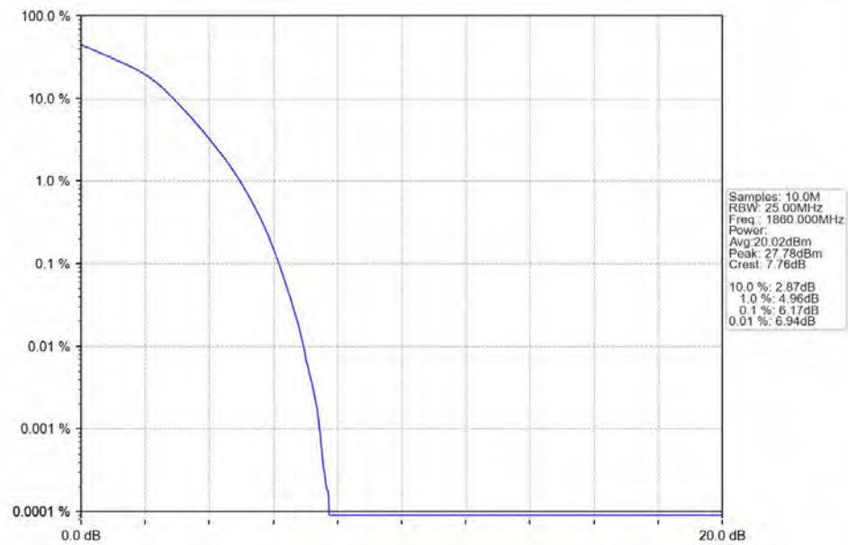
Band25_20MHz_16QAM_LCH_1860MHz_RB_100_0_NTNV
