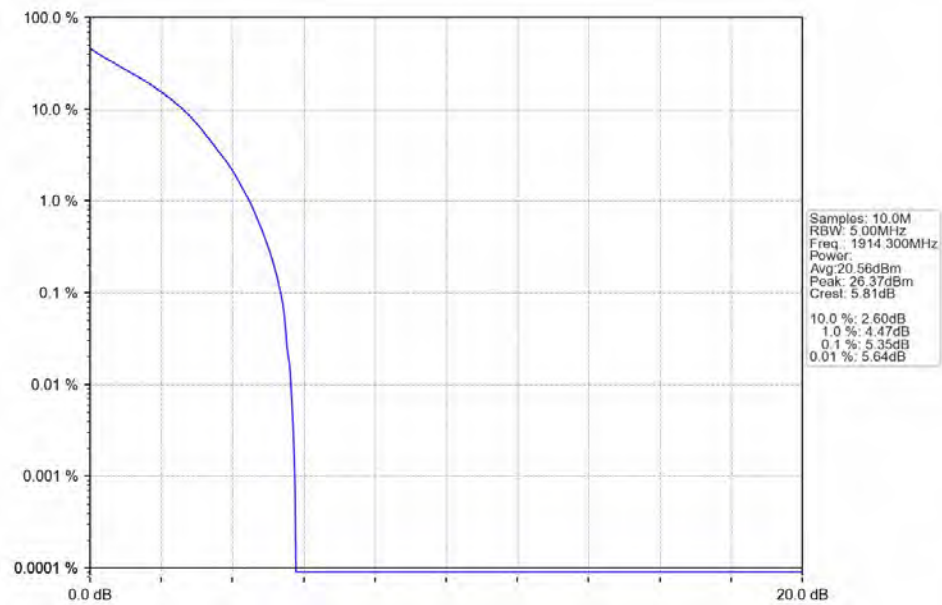
Band25_1.4MHz_QPSK_HCH_1914.3MHz_RB_6_0_NTNV
