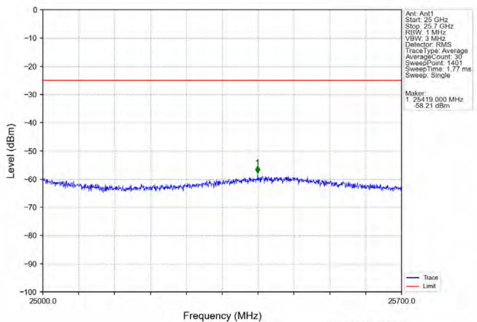
Band7_15MHz_16QAM_HCH_2562.5MHz_RB_1_0_NTNV
